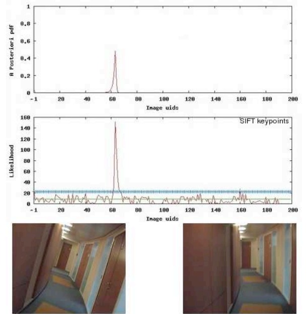
Fig. 6. Another loop-closure detection for the “lip6kennedy” sequence. Although camera orientations are different, the loop-closure is clearly detected as shown by the very peaked a posteriori pdf.
