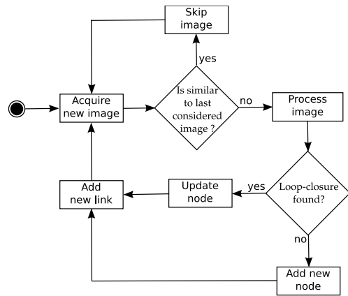
Fig. 1. Overall process diagram (see text for details).
