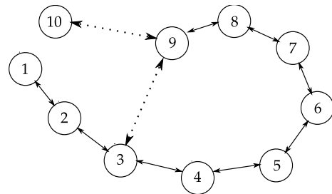
Fig. 2. Time neighboring relations between nodes: in the graph shown here, node 9 is the last added node. When a new image is considered, either a new node will be added (node 10) or an existing one will be updated (node 3). In both cases a new edge connected to node 9 will be added.
