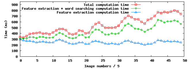
Fig. 7. Evolution of the processing time per image: given is the time needed to extract the features in the images (triangles), to which is added the time required to find the corresponding words in the vocabulary (circles), along with the total computation time per image (squares). The total computation time includes all the processings that lead to the addition or the update of a node in the map (i.e. image processing, word searching, loop-closure probability estimation and multiple-view geometry verification). To enhance readability, computation times have been averaged over 5 images.
