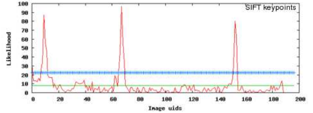
Fig. 6. An example of ambiguous likelihood: this corresponds to a situation where the camera goes back for the fourth time (“d” in figure 5) to an already visited location. From left to right, the peaks correspond to the “a”, “b” and “c” passings of the camera at this location in figure 5. Hopefully, further acquired images will help removing the ambiguity.
