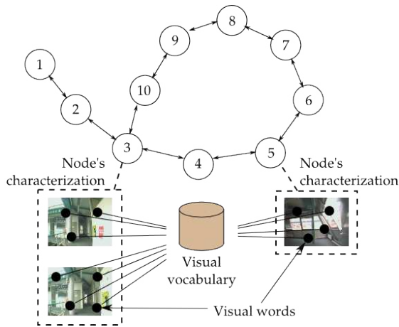
Fig. 3. Illustration of the characterization of the nodes: a node is characterized using the visual words found in the images pertaining to the corresponding location. Since node 3 in the map is a loop-closing node, the visual words from two images are used for its characterization.
