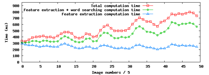
Fig. 7. Evolution of the processing time per image: given is the time needed to extract the features in the images (triangles), to which is added the time required to find the corresponding words in the vocabulary (circles), along with the total computation time per image (squares). The total computation time includes all the processings that lead to the addition or the update of a node in the map (i.e. image processing, word searching, loop-closure probability estimation and multiple-view geometry verification). To enhance readability, computation times have been averaged over 5 images.
