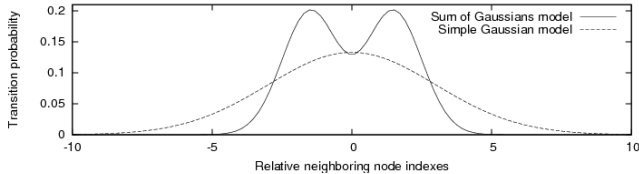
Fig. 4. Sum of Gaussians vs single Gaussian for the time evolution model: the sum of Gaussians model (solid line) gives more emphasis to neighboring states than the single Gaussian model (dashed line), which puts more emphasis to the centre.
