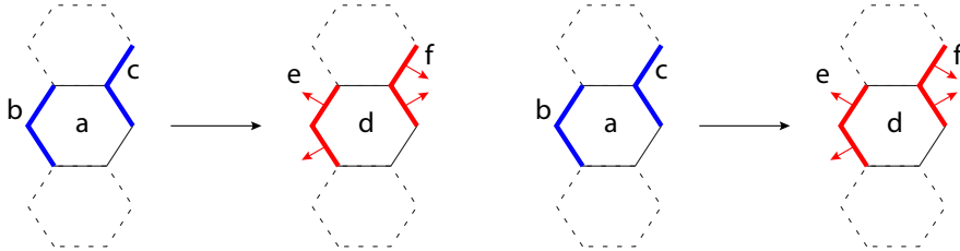
FIG. 5.5. The four local DtN operators
