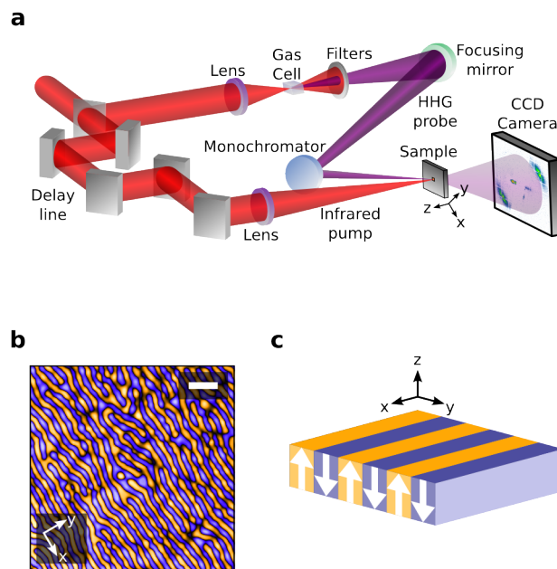
FIG. 1. Set-up and sample characteristics. (a) Schematic diagram of the pump-probe set-up. (b) Magnetic force micrograph of the magnetic structure of the sample, a [Co-Pd] 30 multilayer film. The white scale bar represents 500 nm. (c) This structure consists of alternating up and down magnetic domains aligned along the same direction with an out of plane magnetization (white arrows).
