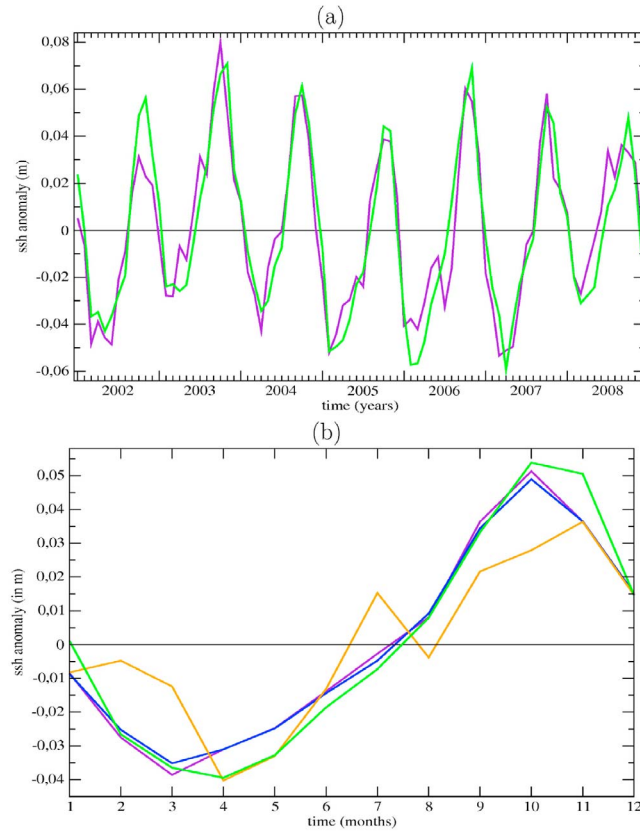
Figure 2. Monthly Sea Surface Height anomaly (m) averaged over the area [11\text{--}7.5^\circ\text{W}, 32\text{--}39^\circ\text{N}] (ABZ in Figure 1a) calculated by subtracting the 2002–2008 SSH mean for each data set. (a) For the period 2002–2008, interannual (84 monthly) values of (purple) GLORYS-1 are compared to (green) AVISO. (b) In average for the period 2002–2008, monthly climatological values are compared between data sets: (blue) MED12-ARPERA, (purple) GLORYS-1 and (green) AVISO. In orange is added the climatological anomalies of SSH which are used in MED12-ARPERA during the 1998–2001 period.
