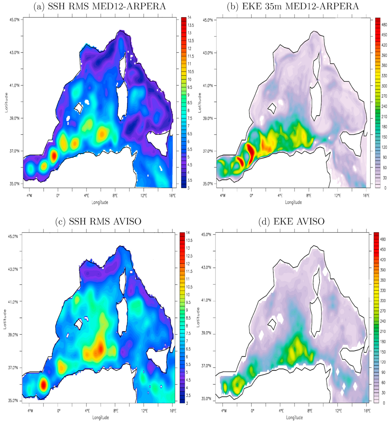
Figure 4. 2004–2008 averages, over the Western Mediterranean, of the RMS of the SSH (SSH Root Mean Square in cm) for (a) MED12-ARPERA and (c) AVISO, and the EKE (Eddy Kinetic Energy in \text{cm}^2\text{s}^{-2} ) for (b) MED12-ARPERA and (d) AVISO. To be consistent with the AVISO geostrophic currents used to calculate the EKE, we took the 35m-depth currents of MED12-ARPERA, i.e., approximately under the mean Ekman layer.
