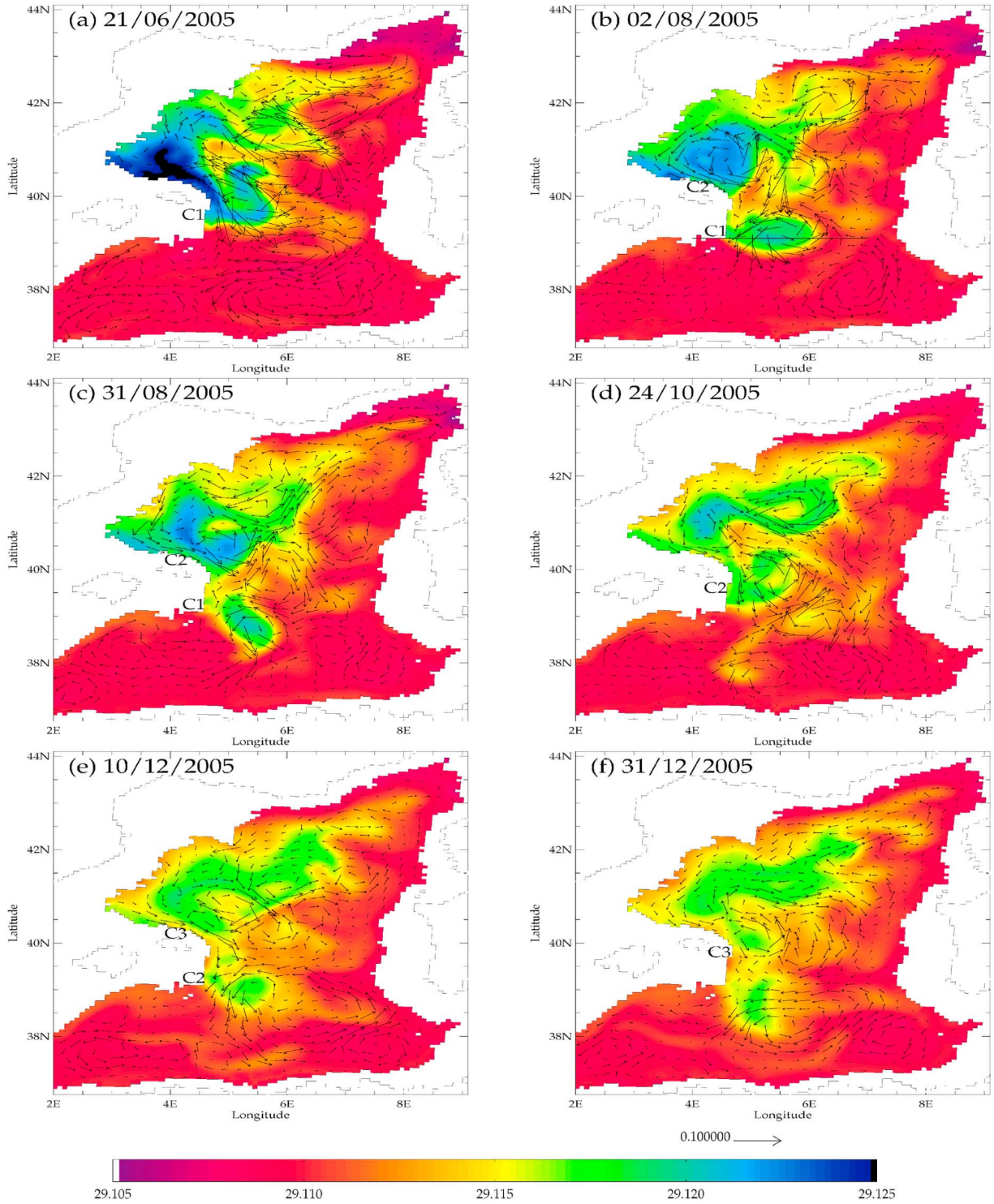
Figure 12. Potential density (colors, in \text{kg.m}^{-3} ) and currents (arrows, in \text{m.s}^{-1} ), at 2225 m depth, for (a) the 21st June 2005, (b) the 2nd August 2005, (c) the 31st August 2005, (d) the 24th October 2005, (e) the 10th December 2005 and (f) the 31st December 2005. One vector in three is plotted. C1, C2 and C3 identify the three successive deep cyclones. The section of Figure 13 is drawn on Figure 12b.
