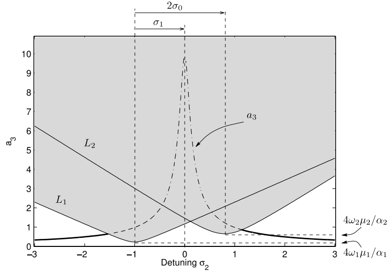
Fig. 12. Stability of the s dof solution with respect to the perturbations caused by the first configuration ( L_1 curve), and by the second configuration ( L_2 curve). The figure is made with \alpha_1 = 7 , \alpha_2 = 5 , \mu_1 = \mu_3 = 0.1 , \mu_2 = 0.2 , Q = 16 , \omega_1 = 4 , \omega_2 = 4.09 , \omega_3 = 8.1 .
