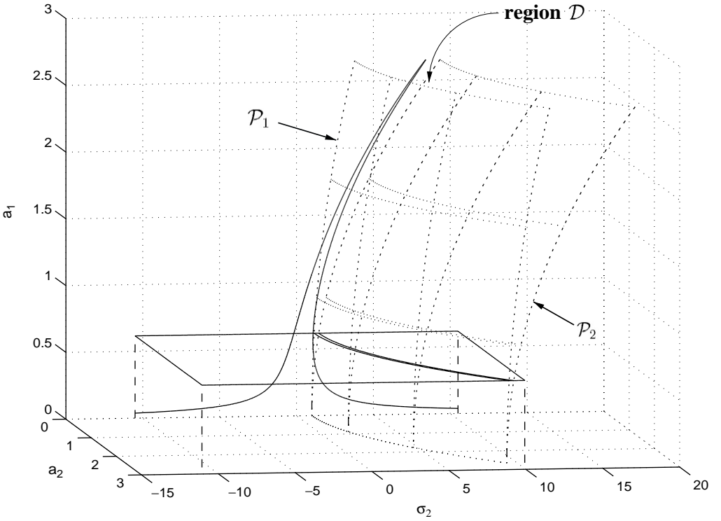
Figure 4. Definition of region ( \mathcal{D} ) in space (\sigma_2, a_1, a_2) where fixed points of dynamical system (40) can exist. The parameters for this figure have been set to the following values: \Gamma_i = C_i = -5 , \mu = 0.15 , \omega_1 = 2\pi , \sigma_1 = 1 . The value of the forcing Q_1 is set to 10. The threshold value defined by equation (43) is represented by the horizontal plane.
