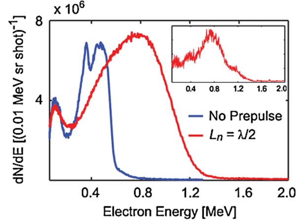
FIG. 3 (color online). Electron spectra measured along the \phi = 36^\circ direction by accumulating 250 laser shots at I \sim 2 \times 10^{18} \text{ W/cm}^2 for the case of no prepulse [blue (dark gray)], and a scale length of \approx \lambda/2 [red (medium gray)]. The inset shows the spectrum from a single laser shot for the optimal scale length of \sim \lambda/2 .
