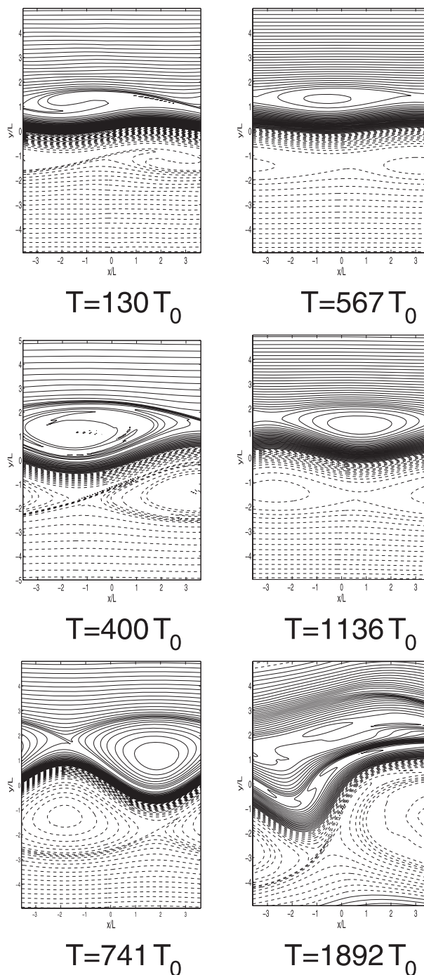
FIG. 14. Nonlinear evolution of PV for the Bickley jet at (left) \lambda = 0.1 and (right) \lambda = 0.5 and Ro fixed at 0.1. The maximum and minimum PV anomaly is \pm 0.15f/(gh_0) for \lambda = 0.1 and \pm 0.5f/(gh_0) for \lambda = 0.5 . The contour interval is 5 \times 10^{-3}f/(gh_0) for \lambda = 0.1 and 2 \times 10^{-2}f/(gh_0) for \lambda = 0.5 .
