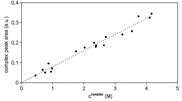
Fig. 4. Variation of the complex peak area with c^{\text{complex}} .
