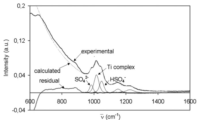
Fig. 2. Representation of the spectra through the deconvolution process.
