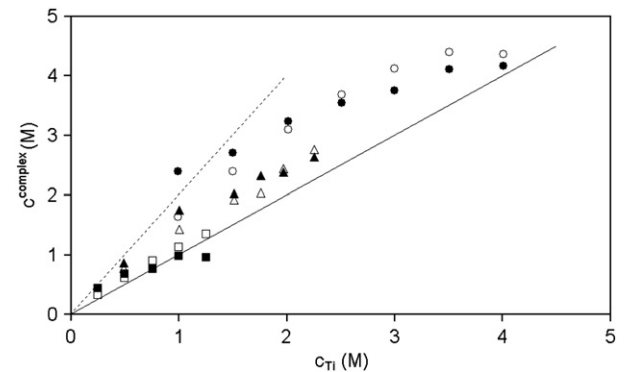
Fig. 5. Variation of c^{\text{complex}} with Ti concentration and c_{\text{H}_2\text{SO}_4}^{\text{apparent}} \approx 2\text{ M} (experimental \blacksquare , calculated \square ), c_{\text{H}_2\text{SO}_4}^{\text{apparent}} \approx 4\text{ M} (experimental \blacktriangle , calculated \triangle ), c_{\text{H}_2\text{SO}_4}^{\text{apparent}} \approx 6\text{ M} (experimental \circ , calculated \circ ).
