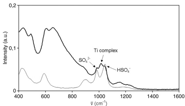
Fig. 1. Effect of Ti(IV) addition on the Raman spectrum of sulphuric acid. — c_{\text{H}_2\text{SO}_4}^{\text{apparent}} = 5.98 \text{ M} and c_{\text{Ti}} = 3.01 \text{ M} , - c_{\text{H}_2\text{SO}_4} = 6.03 \text{ M} and c_{\text{Ti}} = 0 \text{ M} .
