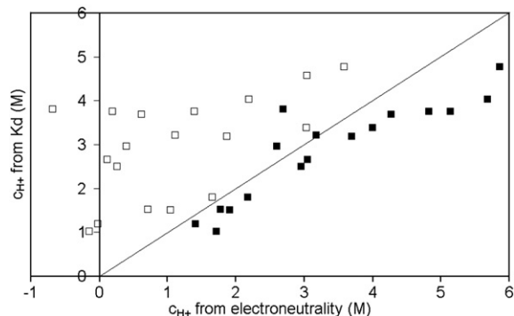
Fig. 6. Comparison between values of c_{\text{H}^+} calculated from \text{HSO}_4^- dissociation constant and from electroneutrality condition, assuming \text{HSO}_4^- complexes ( \square ) or assuming \text{SO}_4^{2-} complexes ( \blacksquare ).
