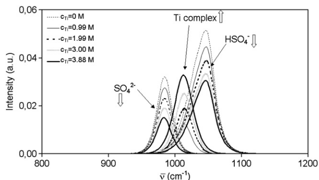
Fig. 3. Changes of Raman spectrum of \text{H}_2\text{SO}_4 solutions for increasing Ti(IV) concentrations at c_{\text{H}_2\text{SO}_4}^{\text{apparent}} \approx 6 \text{ M} .
