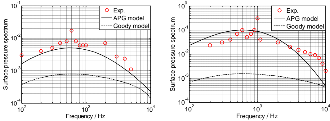
Fig. 2 Wall pressure spectrum measured by Bertagnolio (2012) (circles), and modeled by the APG model (solid line) and Goody's model (dashed line) respectively. Left, U = 30 m/s; right, U = 50 m/s.
