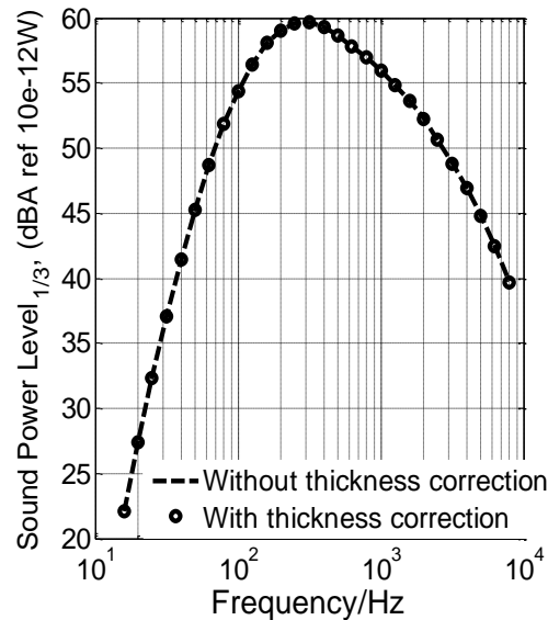
Fig.11 Turbulent inflow noise with/without leading edge thickness correction.
