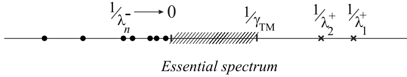
FIGURE 3. Spectrum of A^{-1} .
