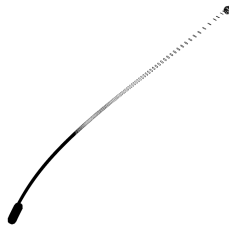
Figure 3.5: Simulation of the Lambert stiff system
