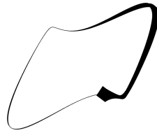
Figure 3.10: Simulation of the vanderpol system ( \mu = 2 )
