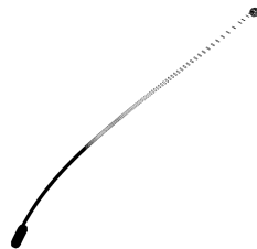
Figure 3.5: Simulation of the Lambert stiff system
