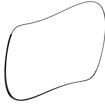
Figure 3.9: Simulation of the vanderpol system ( \mu = 1 )
