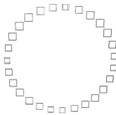
Figure 3.3: Simulation of the circle system
