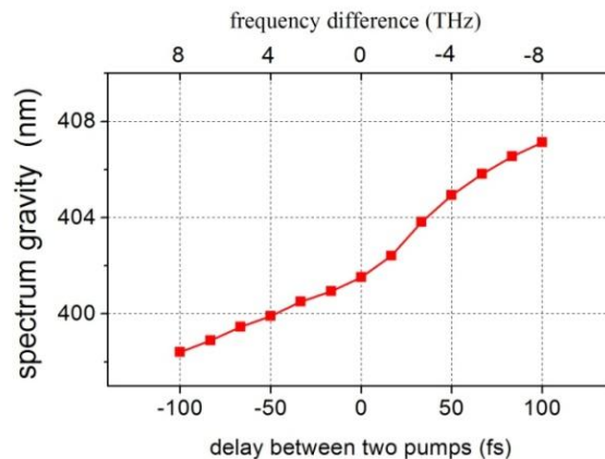
Figure 9. Spectrum center of gravity of the signal pulse as a function of the time delay between the two pump pulses.
