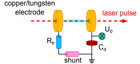
Figure 8. Schematic depiction of the electrical circuit.
