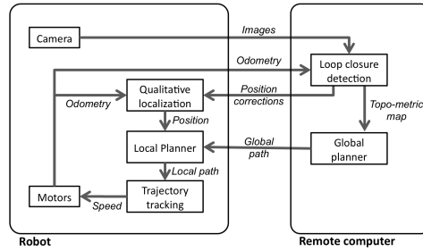
Fig. 9. Simplified diagram of urbi components used by the path following system.
