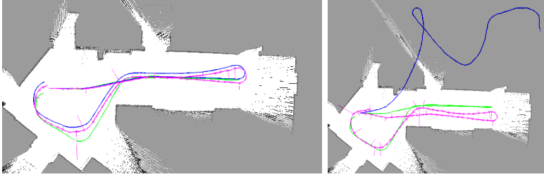
Fig. 16. Two examples of vision based path following using the same map (in green). Raw odometry is in blue, replayed trajectory in magenta. Left: path following using the pioneer 3DX odometry. Right: path following using simulated noise of 6\sigma .
