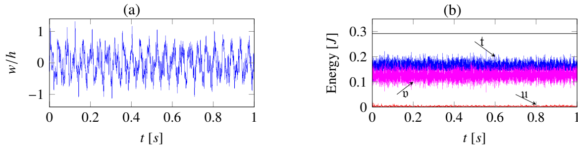
Figure 1: Numerical demonstration of energy conservation. Rectangular undamped plate of lateral dimensions L_x=0.4 m, L_y=0.6 m, thickness h=1 mm, excited by a Dirac delta function of amplitude 1000 N (duration of one sample). (a) : displacement of the plate at \mathbf{x}_0=[0.51L_x \quad 0.11L_y] , normalized by the thickness. (b) Energies. The black continuous and constant thin line is the total discrete energy \mathfrak{h} = \mathfrak{t} + \mathfrak{v} + \mathfrak{u} . Blue thin line (black in BW printing): kinetic energy \mathfrak{t} , magenta thin oscillating line (grey in BW printing) : flexural stored energy \mathfrak{v} . The red thin line oscillating near 0 is the membrane (in-plane) energy \mathfrak{u} .
