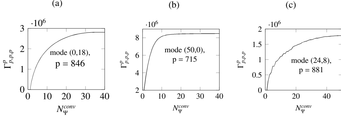
Figure 3: Convergence of nondimensional coupling coefficient \Gamma_{p,p,p}^p as function of the number of in-plane admissible modes N_{\Psi}^{\text{conv}} , for (a) p=846 , axisymmetric mode (0,18); (b) p=715 , mode (50,0); (c) p=881 , mode (24,8).
