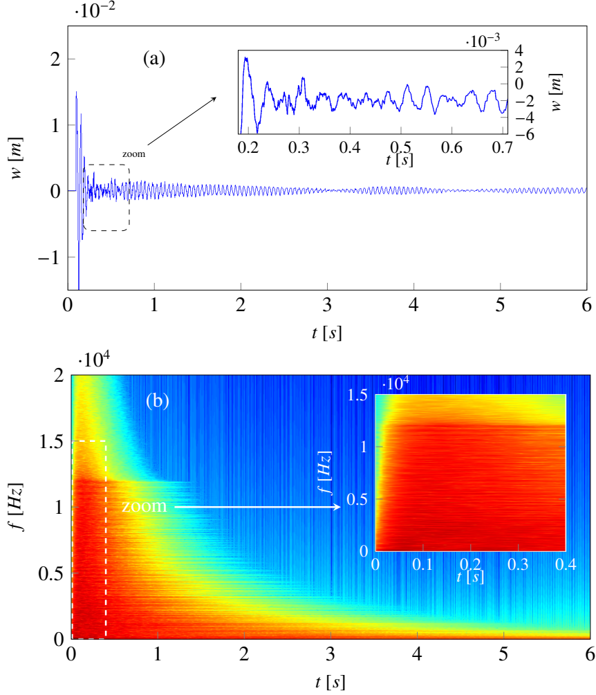
Figure 5: Numerical simulation for the sound synthesis of a cymbal, f_S=80 kHz. Circular plate of radius a=0.2 m and thickness h=0.5 mm, hard impact with T_{wid}=1 ms and amplitude p_m=120 N. (a): time series of displacement at r = 0.896a , with a close-up to observe the high frequencies in the first milliseconds. (b) spectrogram of the velocity at output point.
