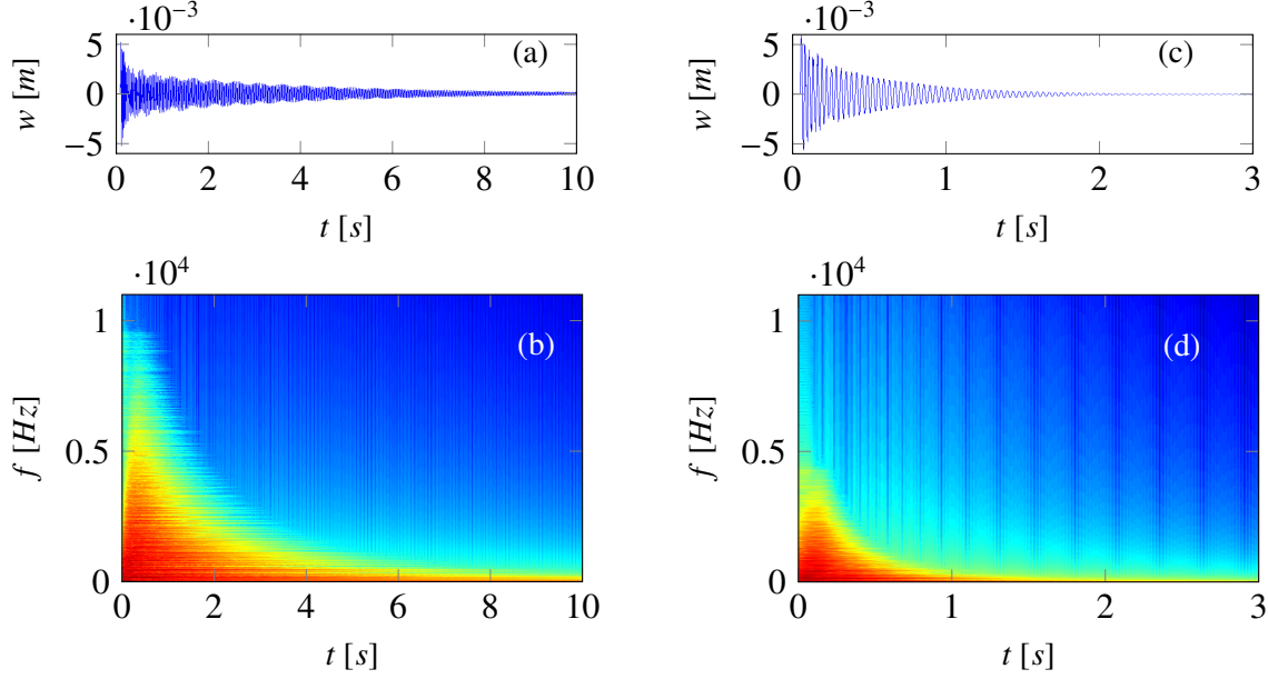
Figure 7: Numerical simulations of a rectangular plate with L_x = 0.4 m, L_y = 0.6 m, h = 1.2 mm. Time series of displacement at output point, spectrograms of velocity at output point, for T_{wid} = 7 ms, p_m = 300 N. Damping law: c = 0.04\omega^{0.75} + 0.08 kg/m 2 /s. (a)-(b): N_\Phi = 500 , N_\Psi = 60 , f_S = 50482 Hz. (c)-(d): N_\Phi = 250 , N_\Psi = 150 , f_S = 25624 Hz.
