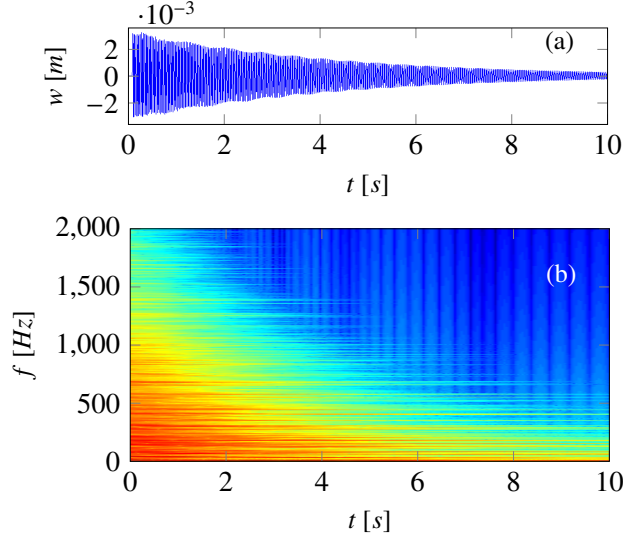
Figure 8: Numerical simulation of a rectangular plate with L_x = 0.4\text{m} , L_y = 0.6\text{m} , h = 1.2\text{mm} , soft strike. (a): Time series of displacement at output point, (b): spectrograms of velocity at output point. T_{wid} = 8\text{ms} , p_m = 80\text{N} , N_\Phi = 100 , N_\Psi = 150 , f_S = 40\text{kHz} , c = 0.004\omega^{0.75} + 0.08\text{kg/m}^2/\text{s} .
