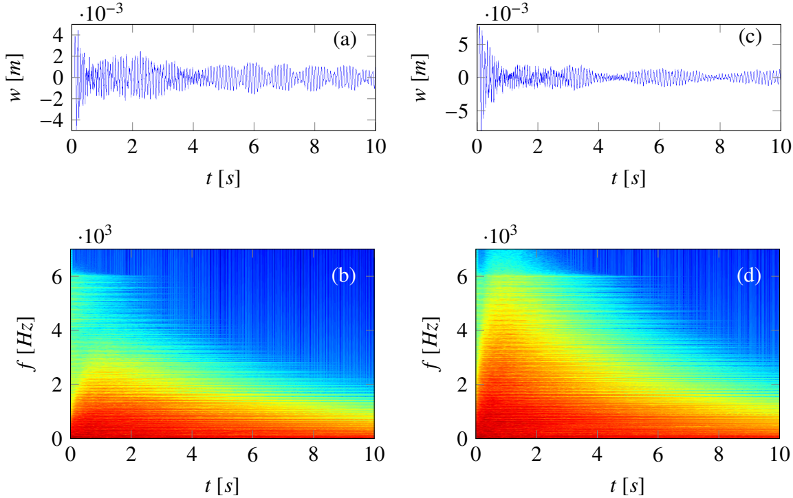
Figure 4: Numerical simulation for the sound synthesis of a gong, f_s=40 kHz. Circular plate of radius a=0.4 m and thickness h=1 mm. (a)-(c): Displacement and (b)-(d): spectrograms of the output point w located at r = 0.896a . Soft strike with T_{wid}=6 ms and (a)-(b): p_m=40 N, (c)-(d): 80 N.
