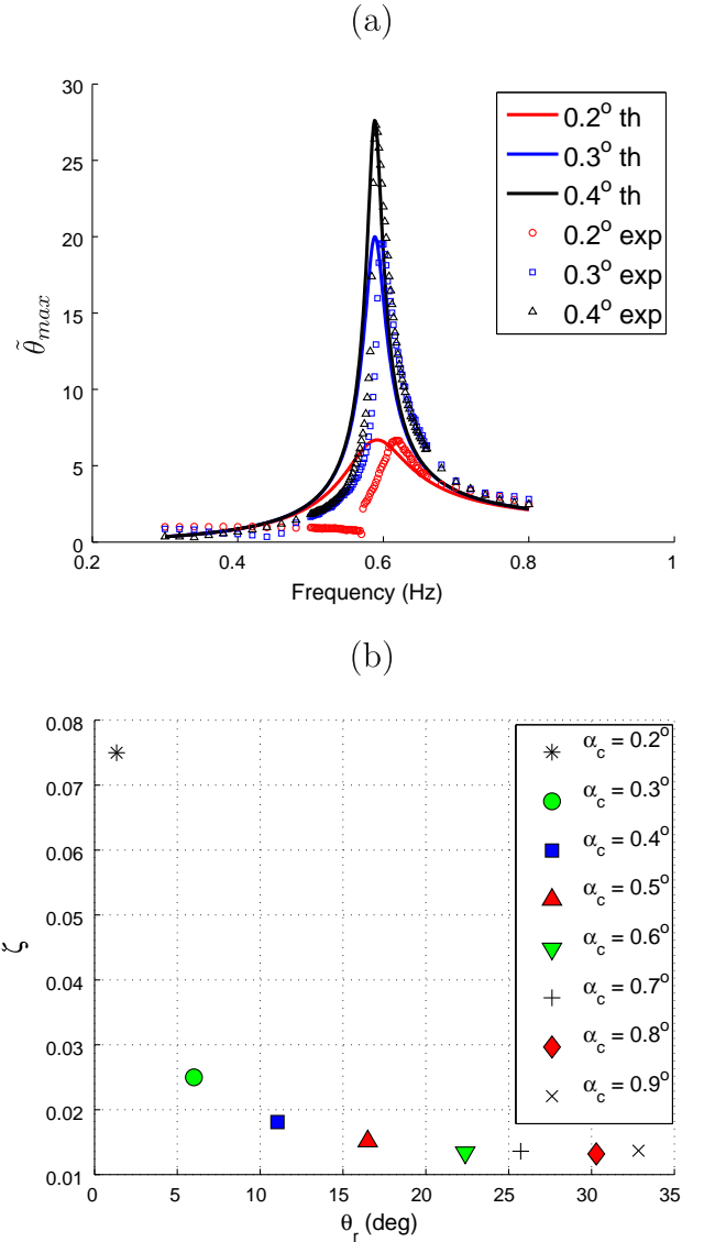
Fig. 10. (a) Experimental normalised frequency response function for three values of \alpha_c compared with the theoretical response function where the damping parameter is adjusted and (b) damping parameter as function of response amplitude.
