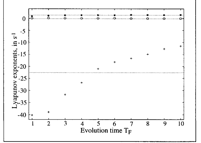
Figure 2. Lyapunov exponents for the Lorenz system, as a function of the evolution time T_F . The optimal value for T_F is T/2 . The calculation has been made with 40000 points from the first coordinate of the Lorenz system, with K = 1500 , d_E = 4 , d_L = 3 , and T = 10 . The true exponents are marked by dotted lines. A quadratic fit has been used. The influence of T_F is particularly visible on the negative exponent (marked by a (+)), whereas the positive one and the vanishing one ((*) and (o)) do not vary significantly with T_F .
