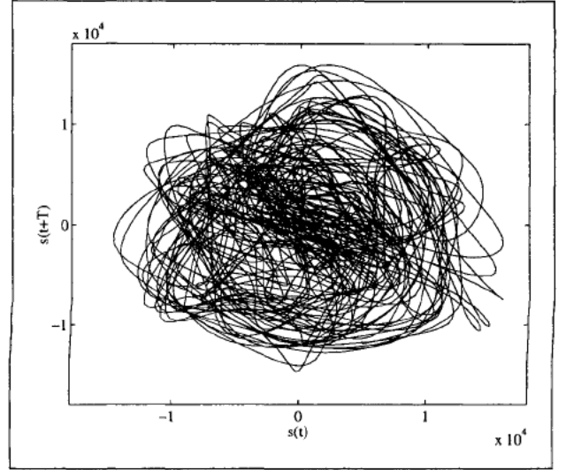
Figure 6. Trajectory in the reconstructed phase space, with T = 16 , for an acceleration signal of the cymbal driven at 526 Hz, once the chaotic regime is established.
