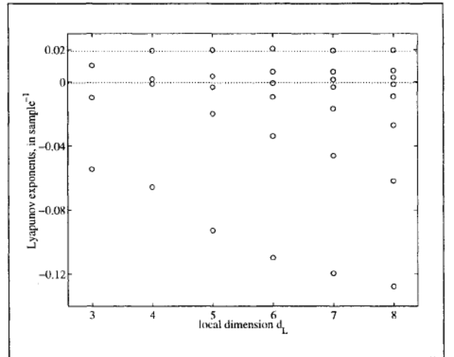
Figure 7. Lyapunov exponents in (\text{sample})^{-1} , as a function of the local dimension d_L , for the acceleration signal recorded at the edge of the cymbal driven with F_{exc} = 526 Hz. 30000 points are used for the analysis. The parameters have the following values: d_E = 8 , K = 2000 , T = 16 , T_F = 10 . A clear convergence to 0.020 is observed for the largest exponent.
