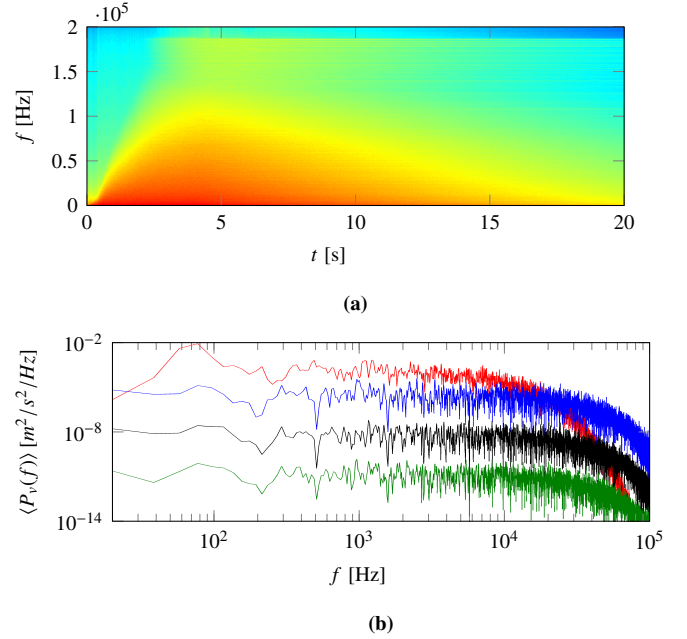
Figure 16: (a): Spectrogram of the velocity for the perfect damped plate. (b): Corresponding velocity power spectra averaged over T = 0.15 \text{ s} computed every 5s from 5 to 20 s).
