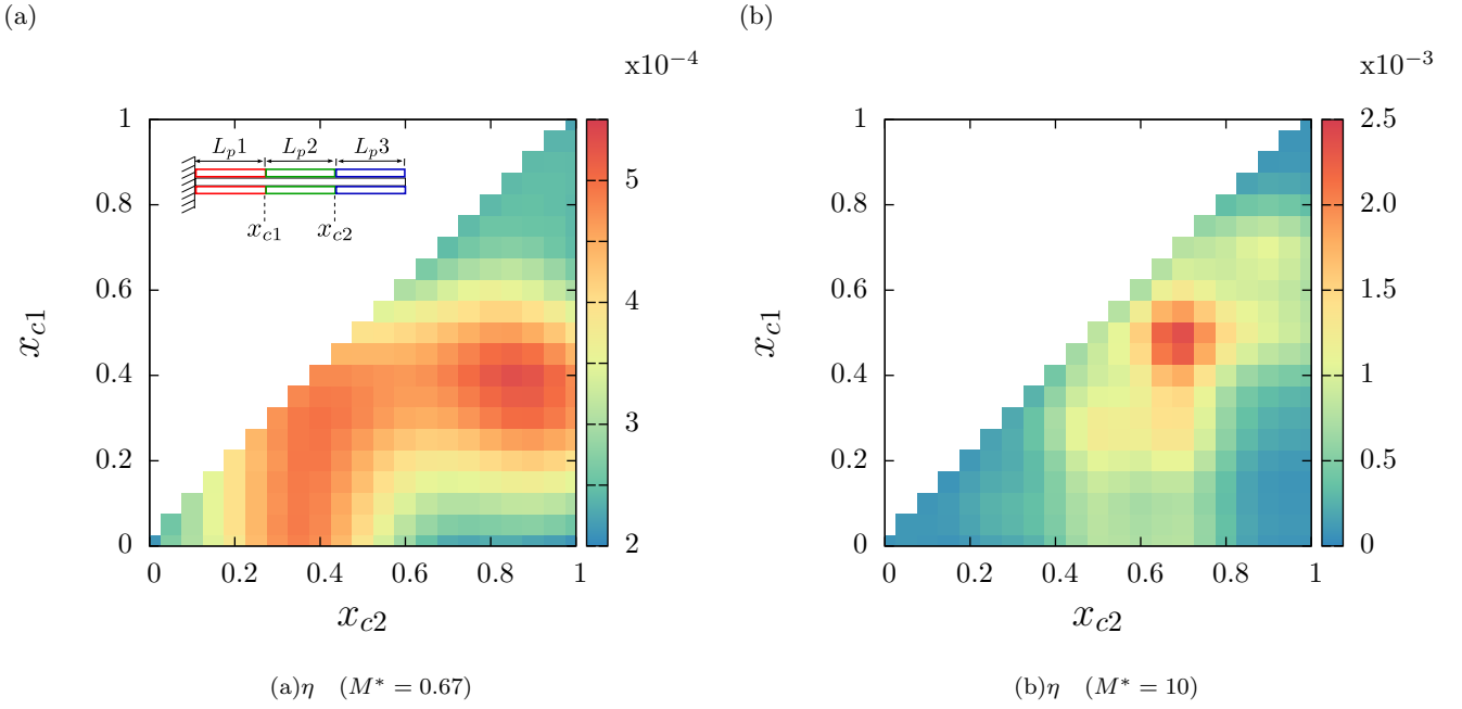
FIG. 12. Energy harvesting efficiency for a piezoelectric plate covered by three electrodes of variables size. (a) : M^* = 0.67 and U^* = 13 . (b) : M^* = 10 and U^* = 8.25 . In both cases \alpha = 0.25 and H = 0.5 .
