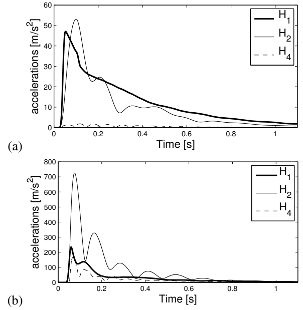
Figure 7. Same measurements than Fig. 6, filtered on harmonics 1, 2 and 4. Evolution of each harmonics with time.
