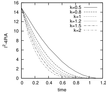
FIG. 6. Isoperimetrical deficit.
