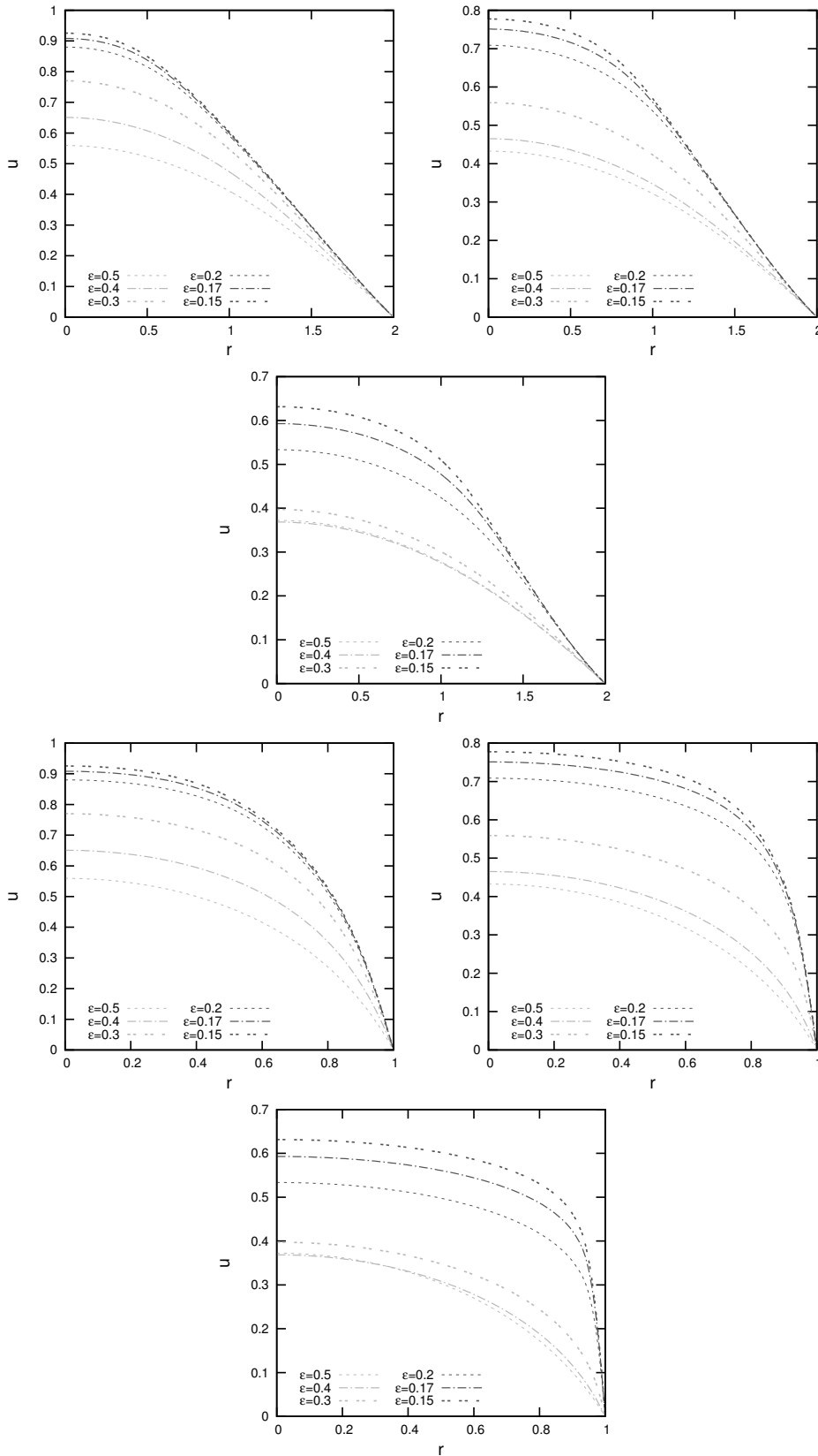
Fig. 6: Solution for ellipse as initial curve. Picture 1–3: Section in direction of the long half axis of the initial curve for k = 1, 1.5, 2 ; Picture 4–6: the same for the short half axis.
