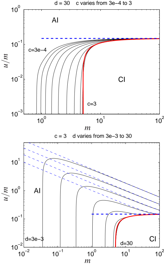
FIGURE 5: Critical curves for transition between convective and absolute instabilities (thin plain line) compared with that given by using g defined in equation (20), thick dashed line, equation (21), thin dashed lines and equation (23), thick solid line.
