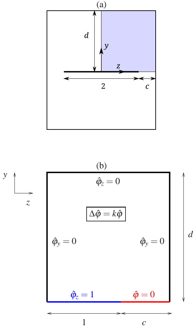
FIGURE 2: (a), complete geometry of the problem in Fourier space; (b), numerical domain and boundary conditions after taking into account symmetries of the problem.
