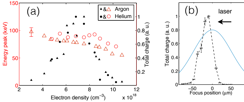
Figure 4. (a) Measured electron beam charge and peak energy over a range of plasma densities. The peak energy is computed from the weighted average energy over a spectral width at 90% of the maximum. (b) Electron charge measured by Lanex signal versus laser focus position relative to the center of the capillary nozzle. Z < 0 means laser is focused on the rear side of the nozzle. The blue line is the shape of a Gaussian density profile with a FWHM of 120 \mu\text{m} .
