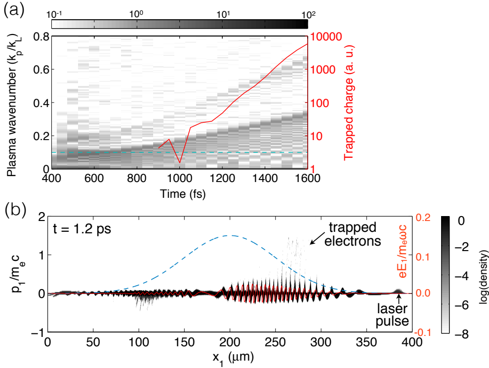
Figure 5. (a) The evolution of plasma wave number spectrum from the 3D PIC simulation. Solid curve (red) is the total charge of the trapped electrons defined as those with p_e/m_e c > 0.2 which corresponds to a kinetic energy of about 10 keV. (b) The electron momentum phase-space ( x_1, p_1 ) at t = 1.2 ps. Dashed curve (blue) is a lineout of the Gaussian density profile. Solid curve (red) is the normalized on-axis longitudinal electric field E_1 . The laser travels from left to right.
