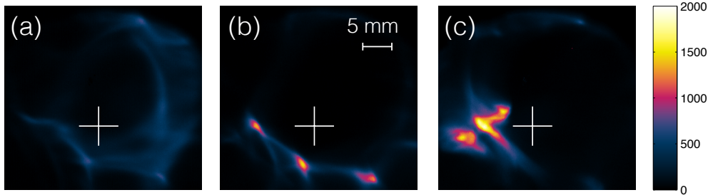
Figure 2. Typical electron beam profiles (from argon plasma) measured at 32 cm downstream. The white cross indicates the position of the laser propagation axis. The length of each arm represents a half angle of 10 mrad. These three images were taken under the same experimental conditions except the deformable mirror is (a) off (a “flat” mirror); (b) optimized for best SHG generation and (c) optimized for best electron signal. The acquisition time are 1000 ms, 1000 ms, and 200 ms respectively for (a), (b) and (c).
