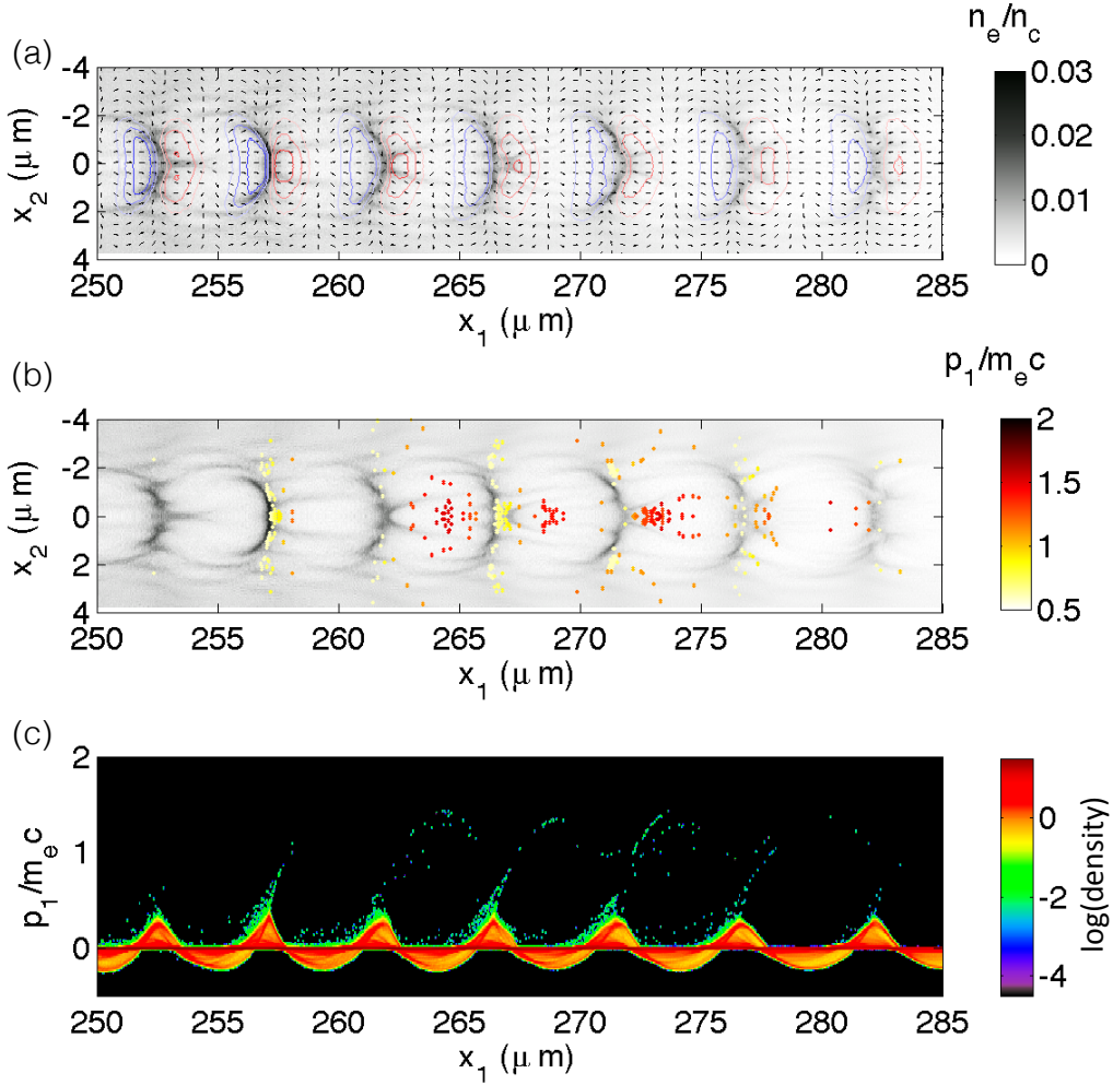
Figure 6. Simulation results from 2D PIC at 1.2 ps in the trapping region (zoomed) of figure 5(b). The laser travels from left to right. (a) Electron density and electric field in space x_1 - x_2 . Black arrows represent the electric field direction. The magnitude of longitudinal electric field E_1 is indicated by the isocontours, where the red (blue) colour corresponds to an accelerating (decelerating) field for electrons. (b) Spatial distribution of the accelerated electrons in x_1 - x_2 . Colour represents the electron longitudinal momentum p_1 . (c) Electron phase space (x_1, p_1) .
