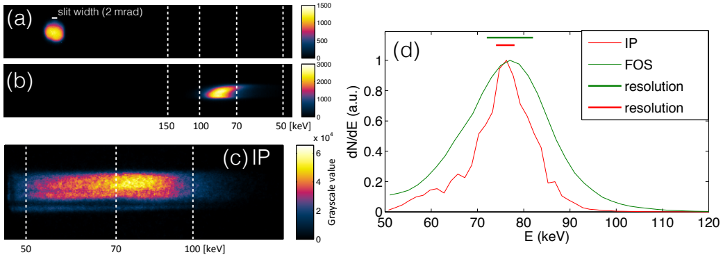
Figure 3. (a)(b): Typical spectrum data obtained with FOS plate (from argon plasma) (a) without magnets (no slit; electron beam through the pinhole) (b) spectrally dispersed electron. (c) Raw spectrum data on image plate with the custom-built electron spectrometer under the same experimental conditions as in (b). (d) Deconvoluted electron spectra for (b) and (c) using calibrated detector response for both FOS and IP. Each horizontal bar represents the energy resolution due to the finite acceptance angle from the slit or the pinhole.
