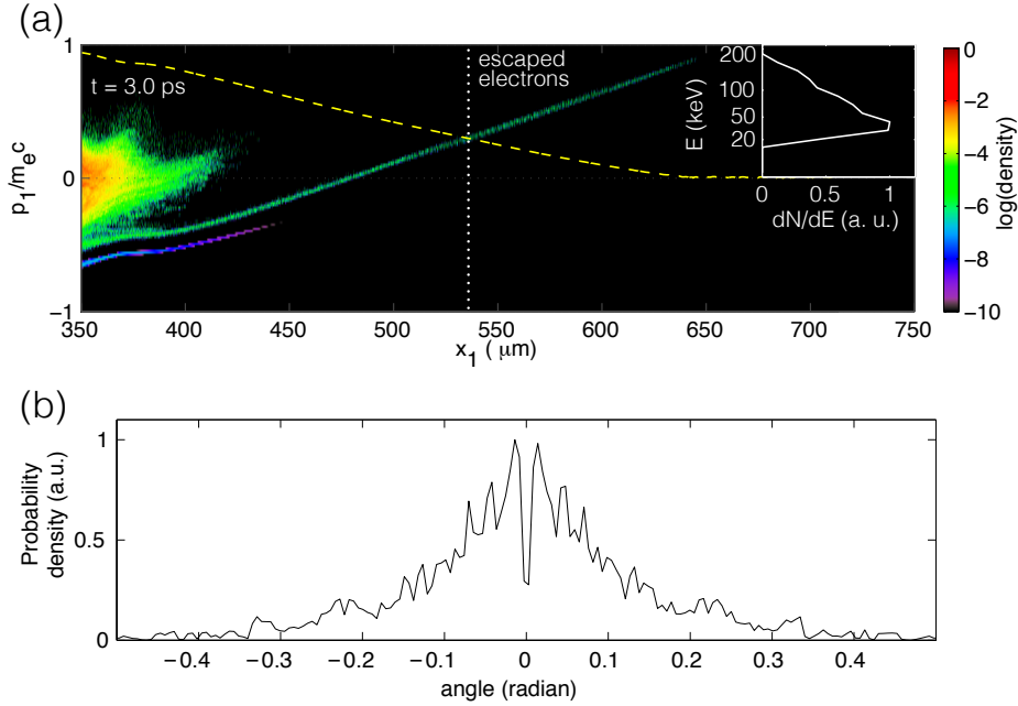
Figure 7. (a) The electron phase space (x_1, p_1) at t = 3.0 ps. Dashed curve (yellow) is the plot of the additive inverse of the longitudinal electric potential expressed in \text{sgn}(\phi)\sqrt{(|\phi|/m_e c^2 + 1)^2 - 1} . The energy distribution of the escaped electrons defined as those with E + \phi > 0 is shown in the inset. (b) Angular distribution of the escaped electrons in the simulation.
