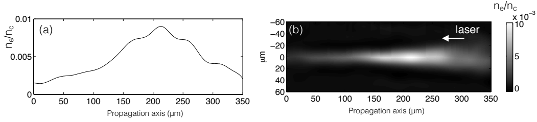
Figure 1. (a) Lineout of electron on-axis density. (b) Reconstructed electron density map.
