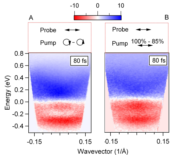
FIG. 4: A: Map of the dichroic contrast acquired at delay time of 80 fs and generated by switching the circular polarization of the pump beam. B: Difference between the photoelectron intensity maps acquired with pump fluence of 30 \mu\text{Joule}/\text{cm}^2 (reference fluence) and 25 \mu\text{Joule}/\text{cm}^2 (85% of the reference fluence) at delay time of 80 fs.
