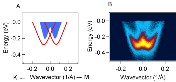
FIG. 1: A): Calculated band structure of the Te terminated BiTeI surface for parallel wavevector along \Gamma -K and \Gamma -M. B): Photoelectron intensity map acquired along the \Gamma -K direction with photon energy of 28 eV.
