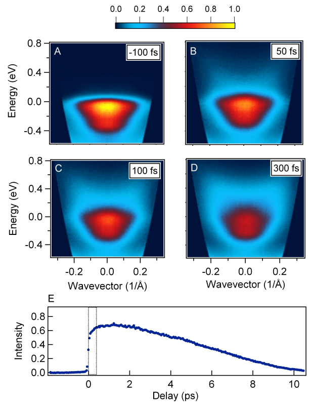
FIG. 2: A-D): Photoelectron intensity maps acquired along \Gamma -K for different pump probe delays. E): Photoelectron intensity at 0.15 eV above the Fermi level as a function of pump-probe delay. The dashed lines indicate the temporal window of the electronic thermalization.
