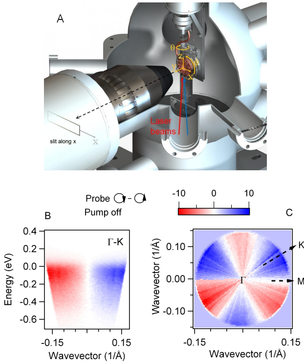
FIG. 3: A: Experimental geometry of our experimental setup. The electrons are detected in the incident plane of the laser beams ( xy plane). Both the pump and probe beams define an angle of 45^\circ with respect to the surface normal. B: Dichroic map generated by switching the circular polarization of the probe beam and integrating the electronic states in an acceptance window of 0.2 eV centered at -0.1 eV. C: Map of dichroic contrast generated by the probe beam along the \Gamma -K direction. These data have been acquired without pump beam.
