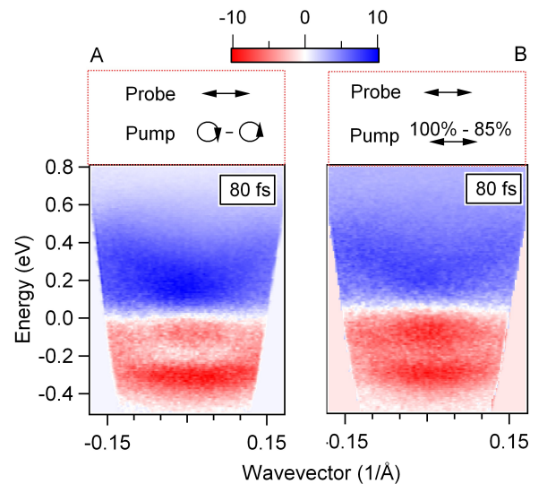
FIG. 4: A: Map of the dichroic contrast acquired at delay time of 80 fs and generated by switching the circular polarization of the pump beam. B: Difference between the photoelectron intensity maps acquired with pump fluence of 30 \mu\text{Joule}/\text{cm}^2 (reference fluence) and 25 \mu\text{Joule}/\text{cm}^2 (85% of the reference fluence) at delay time of 80 fs.
