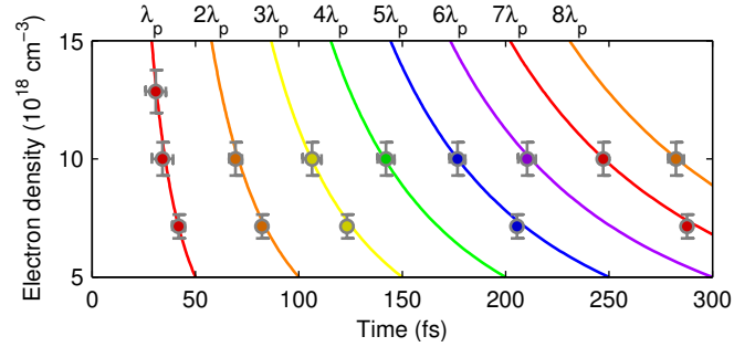
Figure 4. (Color online) Average positions of the Fourier peaks for different plasma densities (o) are compared to multiples of the plasma wave period (lines). Horizontal errorbars denote the standard deviation over the complete dataset. Vertical errorbars is an estimate of the uncertainty in plasma density.
