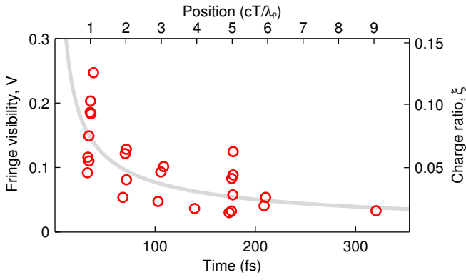
Figure 3. (Color online) Fringe visibility for sinusoidal oscillation that contained only one significant peak in the Fourier Transform, as function of the position of that peak. The charge ratio \xi = q_n/q_o is calculated from the visibility using Eq. 2 in the limit where both bunches have similar shapes and energy distributions. The measurements were performed using CPI for n_e = 10 \times 10^{18} \text{ cm}^{-3} .
