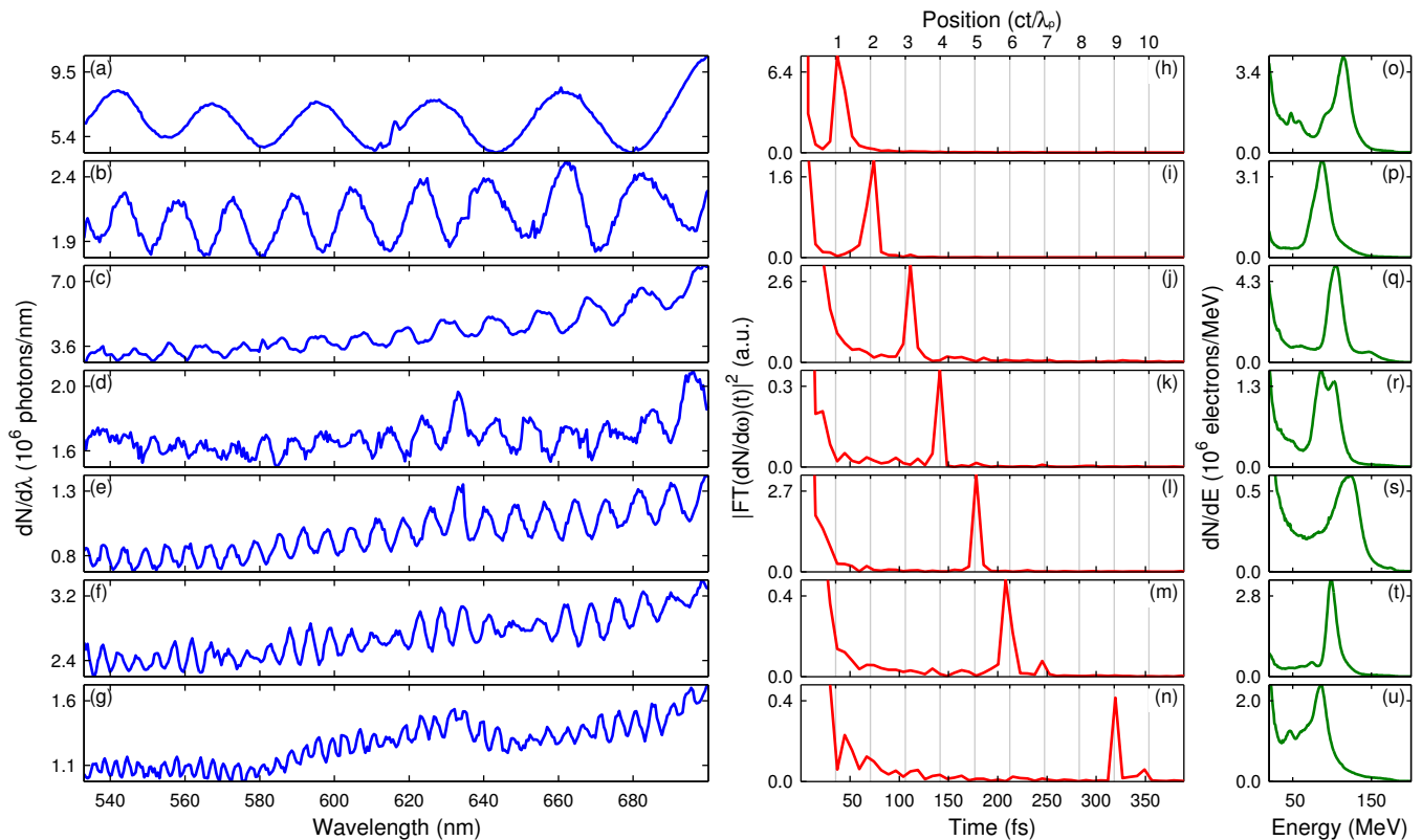
Figure 1. (Color online) Selected and sorted examples of sinusoidal CTR modulations, obtained using CPI for n_e = 10 \times 10^{18} \text{cm}^{-3} and \lambda_p = 10.6 \mu\text{m} . Three panels on each row represent one measurement. (a–g): CTR spectra. (h–n): Square amplitude of the Fourier transform of the CTR spectra. (o–u): Corresponding electron spectra.
