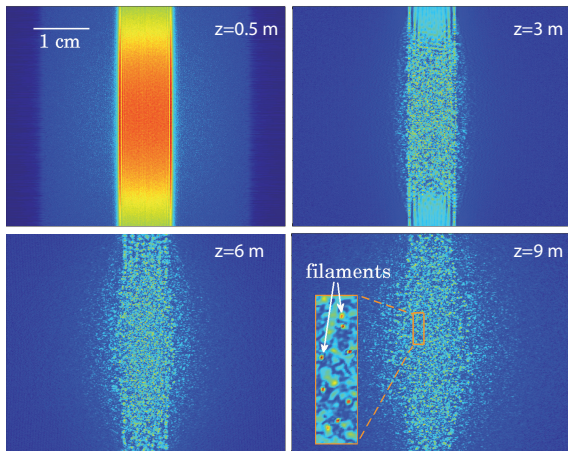
FIG. 7. Simulated beam intensity cross sections along propagation for a collimated cw beam under distortion of the slit mask. Absence of beam symmetrization and of filament density increase are evident (compare with Fig. 3(b)). Numbers in figures mark propagated distances along z . The reference Gaussian pulse used in this modeling is of 100 fs and the input beam peak intensity is 2.5 \text{ TW/cm}^2 . All figures have a cross-section of 4 \times 4 \text{ cm}^2 .
