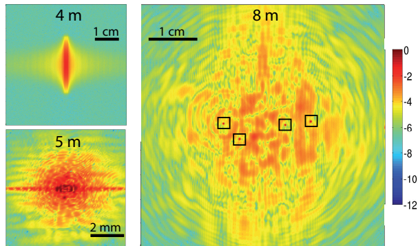
FIG. 5. Beam symmetrization in the low filament limit. Logarithmic scale plots of beam Intensity profiles at various propagation distances (see labels) for a beam focused with a lens of 5 m of focal length and perturbed with a 10 \times 35 \text{ mm}^2 slit mask (as in Figs. 3 and 4). Input peak intensity I_0 = 50 \text{ GW/cm}^2 . All nonlinear effects of Eq. 1 are switched on ( n_2, \beta_8, \sigma \neq 0 ).
