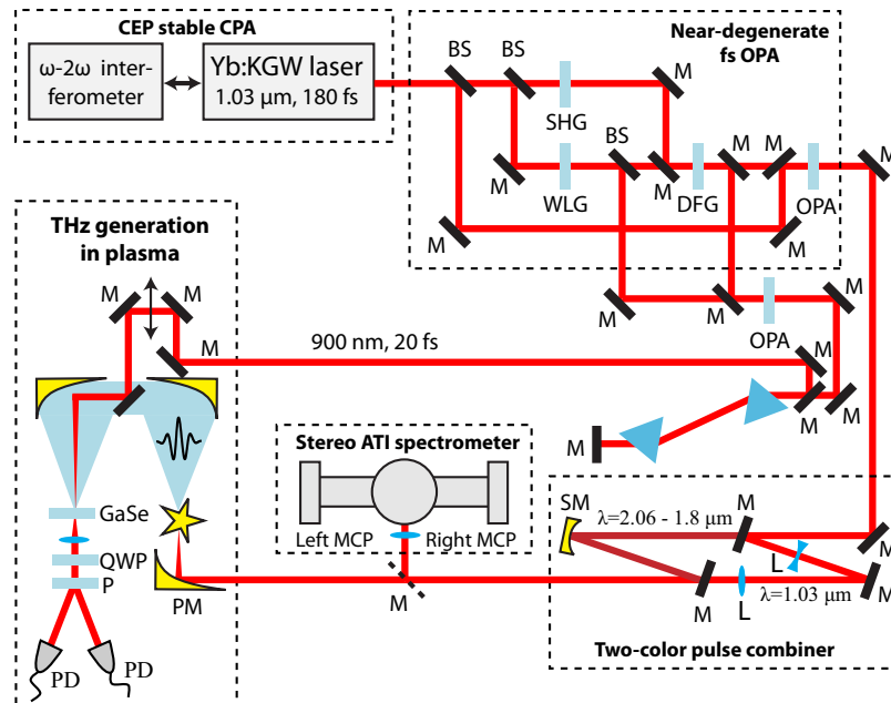
Fig. 4. Scheme of the experimental setup. THz emission was detected via electrooptic (EO) sampling setup based on GaSe crystal. The probe pulses were generated in an additional OPA and compressed down to 20 fs in a prism compressor.
