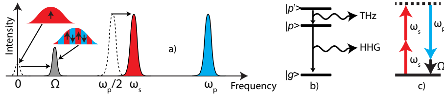
Fig. 1. (a) Scheme of mixing two incommensurate frequencies for generating tunable THz emission. (b) Scheme of the atomic transitions in a strong laser field: transitions between a continuum and a ground state yield HHG, while transitions between continuum states yield low order harmonic generation (including THz). (c) Perturbative four-wave mixing scheme for THz generation.
