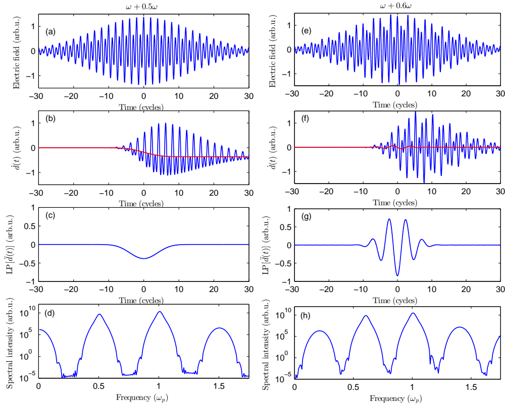
Fig. 2. Simulation of the induced current, using Eqs. (6)–(9) with \Gamma(t_b) = \exp[-2(2I_p)^{3/2}/(3|F_{\text{las}}(t_b)|)] and the classical expression \bar{v}(t, t_b) = -\int_{t_b}^t F_{\text{las}}(t') dt' , for two-colour fields with two frequency ratios: the left and right-hand sides correspond to the commensurate and incommensurate frequency case, respectively. Shown are the considered driving electric fields (first row), the dipole velocity (Eq. (6)), corresponding to the induced current (second row, blue line; the red line shows a low-pass filtered version), the low-pass filtered (retaining only the THz-sideband) dipole acceleration (Eq. (8)), corresponding to the emitted THz-near-field (third row), and the spectral intensity of this emission (square of Eq. (9)) (fourth row). The considered ionization potential is that of nitrogen molecules, I_p = 15.7 eV. The \omega_p -component of the driving field has a peak field strength of F_{\text{max}} = 27 GV/m (corresponding to 1 \times 10^{14} W cm ^{-2} ), and the \omega_s -component has F_{\text{max}} = 13.5 GV/m and a relative phase of \pi/4 .
