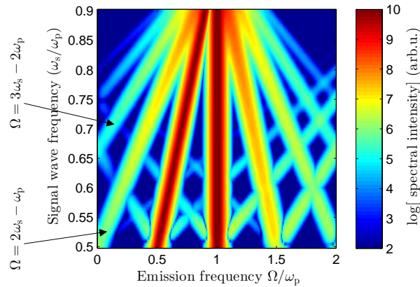
Fig. 3. Simulated power spectrum of the emission (square of Eq. (9)) as a function of the frequency \omega_s of the tunable signal wave, for the same conditions as in Fig. 2.
