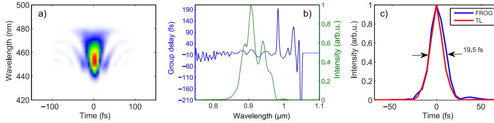
Fig. 6. Temporal characterisation of EO sampling probe pulse using SHG FROG. a) measured FROG trace, b) reconstructed spectrum and group delay of the pulse c) measured temporal profile and calculated Fourier limit.
