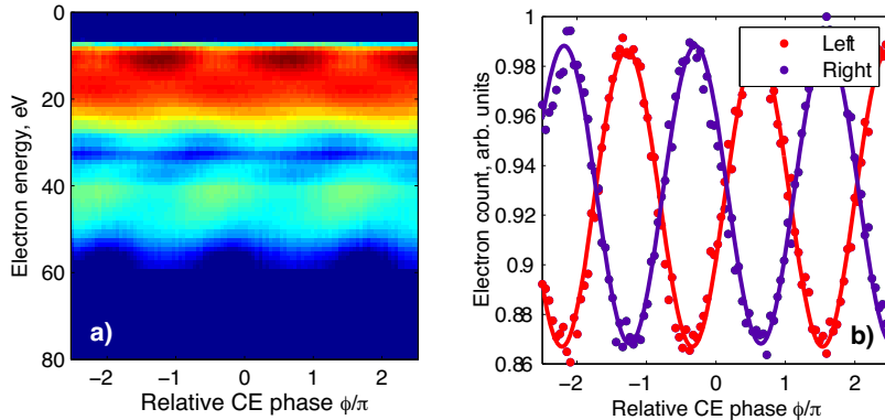
Fig. 5. Stereo-ATI electron spectrometry measurement results obtained with two commensurate-frequency pulses: \lambda_p = 1.03 \mu\text{m} and \lambda_s = 2.06 \mu\text{m} . (a) Electron energy spectrum (log scale) measured on one side of the stereo-ATI spectrometer as function of the fundamental laser CEP. (b) Total electron count in left and right directions of the stereo-ATI spectrometer obtained by integrating the electron spectrum of the left and right detectors.
