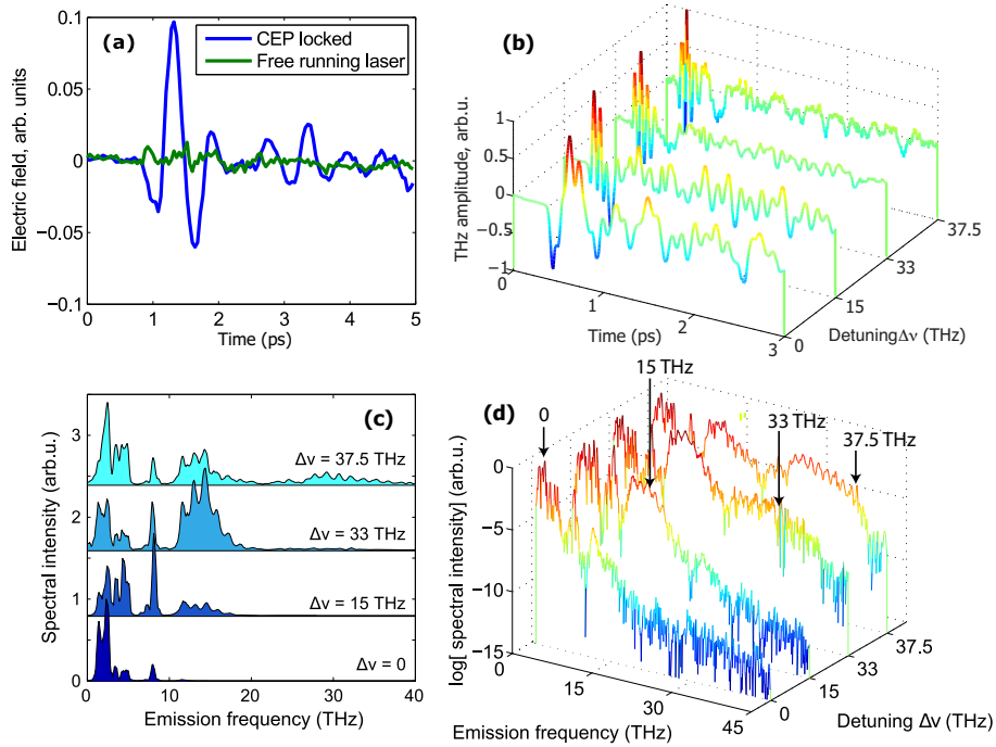
Fig. 7. Experimental THz-generation results with \omega_p + \omega_s two-colour driving fields ( \omega_s = (\omega_p + \Delta\nu)/2 ), for various detunings \Delta\nu , created by combining the fundamental wave ( \lambda_p = 1.03 \mu\text{m} , 250 \mu\text{J} ) with the tunable signal wave ( \lambda_s = [2.06, 1.96, 1.84, 1.80] \mu\text{m} , 20 \mu\text{J} ). (a) Electric field of the THz transient measured using EO sampling in case of locked CEP or free running laser, for zero detuning, \Delta\nu = 0 , i.e. exactly commensurate frequency ratio. (b) Temporal traces of the EO sampling signal for different detunings \Delta\nu , (c) THz emission spectra of plasma calculated from the EO signal, represented on linear scale. (d) The same spectra as in (c), represented on logarithmic scale. Each spectrum and temporal trace was normalised to its maximum. The arrows in panel (d) show the theoretically predicted central frequency of the emission.
