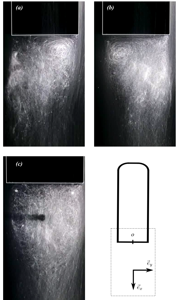
FIG. 12: Flow visualization performed in a water tunnel using bubbles appearing white against a black background. The flow Reynolds number is Re = 216000 at a ground clearance C^* = 0.1 . The drawing shows the visualization area depicted by a dashed rectangle at the rear of the Ahmed body. The obturation time of the camera is \tau^* = 3 , say 3 times larger than the convective time H/U_0 and captures the dynamics at this timescale. In (a), RSB mode of the branch y_b^+ , in (b) its mirror counterpart: the RSB mode of the branch y_b^- . Wake controlled with a vertical control cylinder (diameter d^* = 0.107 ).
