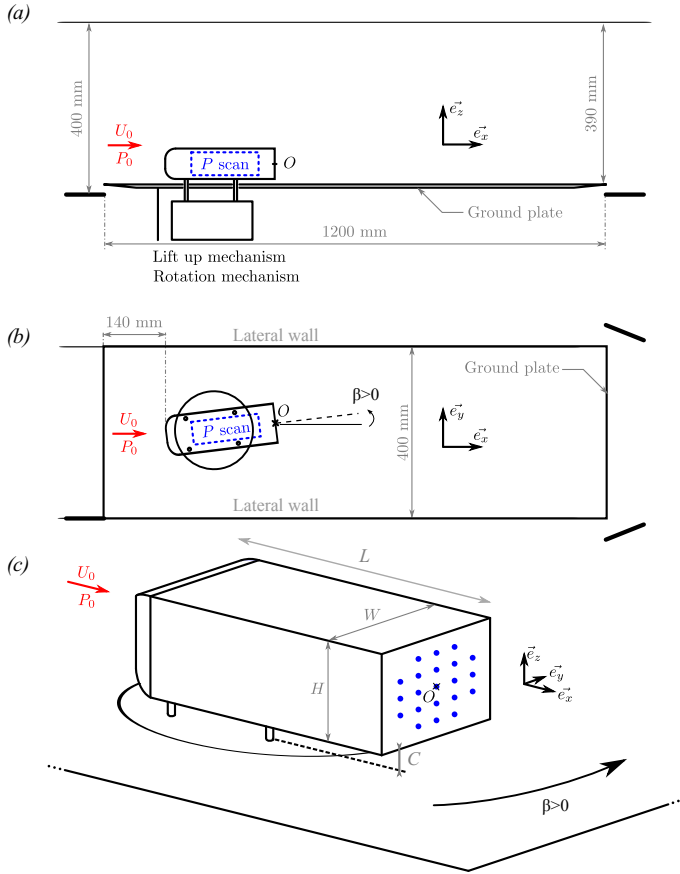
FIG. 1: Experimental setup: side view (a), top view (b) and perspective view (c); the point O at the centre of the body base sets the origin of the coordinate system. The blue dots locate the visible pressure taps; P scan refers to the pressure scanner.
