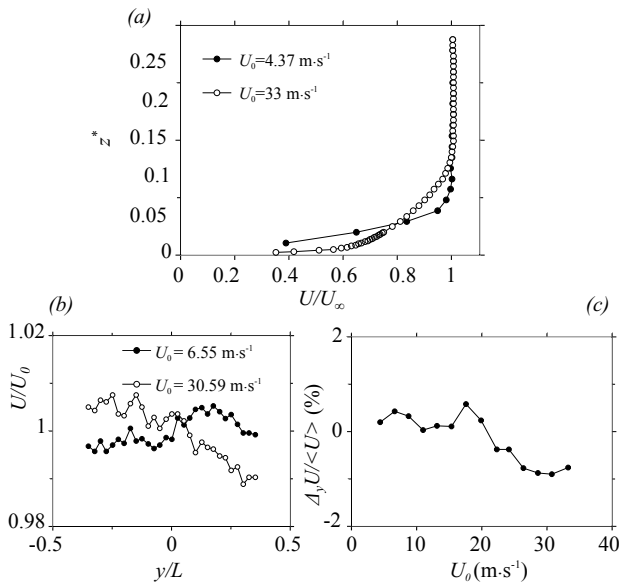
FIG. 2: Free stream characterization at the location of the Ahmed body, boundary layer profile on the floor(a), lateral velocity profile at z^* = 1/2 (b), right to left asymmetry (see text) of the lateral velocity profile vs. the main velocity (c).
