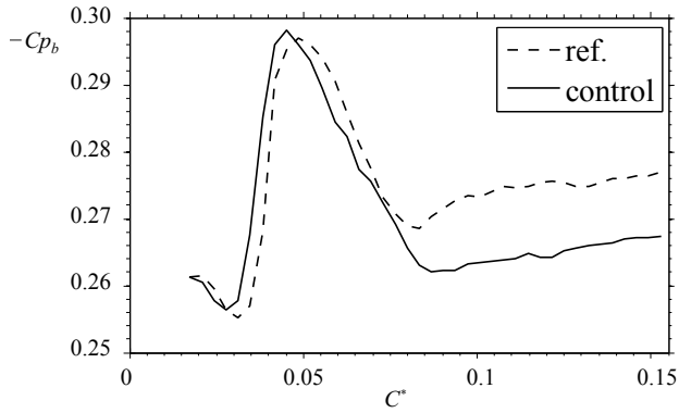
FIG. 11: Base pressure suction vs. the ground clearance for (dashed line) the reference case of Fig. 10(a) and for (continuous line) the controlled case of Fig. 10(b).
