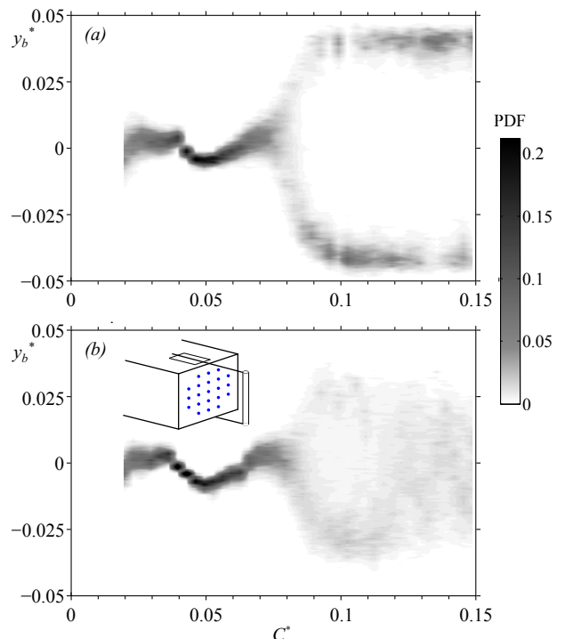
FIG. 10: Probability density functions, PDF(y_b^*) in grey levels for U_0 = 30.58 \text{ m}\cdot\text{s}^{-1} vs. the ground clearance C^* , for (a) with the yaw angle \beta = -0.4^\circ and (b) with a yaw angle \beta = +0.4^\circ . The white lines represent the most probable position and correspond in (a, continuous line) to the stable branch y_b^{*+} and in (b, dashed line) to the other stable branch y_b^{*-} .
