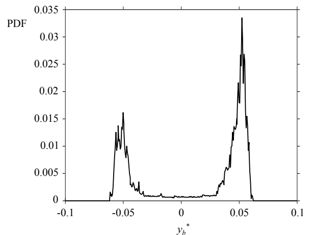
FIG. 4: Probability density function (PDF) of the horizontal coordinate y_b^* of the base pressure barycenter computed from the time series in Fig. 3(c).
