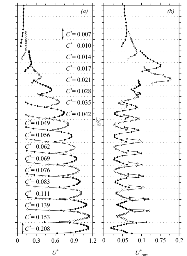
FIG. 6: Characterization of the underbody flow using hot wire anemometer measurements, 2 mm behind the body in the y = 0 plane. The hot wire is oriented to be sensitive to the longitudinal velocity u(t) . (a) : z/C vs. the time averaged non-dimensional velocity U^* = \bar{u}^* . (b) Fluctuating velocity defined as U_{rms}^* = \sqrt{(u^* - U^*)^2} .
