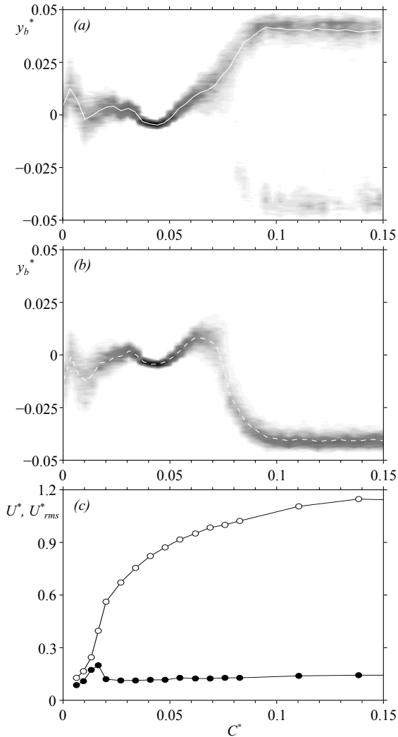
FIG. 7: Probability density functions, \text{PDF}(y_b^*) in grey levels for U_0 = 30.58 \text{ m}\cdot\text{s}^{-1} vs. the ground clearance C^* , for (a) with the yaw angle \beta = -0.4^\circ and (b) with a yaw angle \beta = +0.4^\circ . The white lines represent the most probable position and correspond in (a, continuous line) to the stable branch y_b^{*+} and in (b, dashed line) to the other stable branch y_b^{*-} . In (c) are reported the maximum of the profiles measured in Fig. 6, mean velocity U^* (empty circles) and fluctuation U_{rms}^* (black filled circles).
