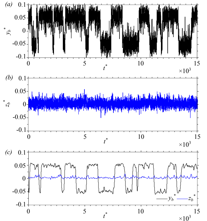
FIG. 3: Time series of the base pressure barycenter coordinates ( y_b^* , z_b^* ), y_b^* (a), z_b^* (b) and filtered in (c).
