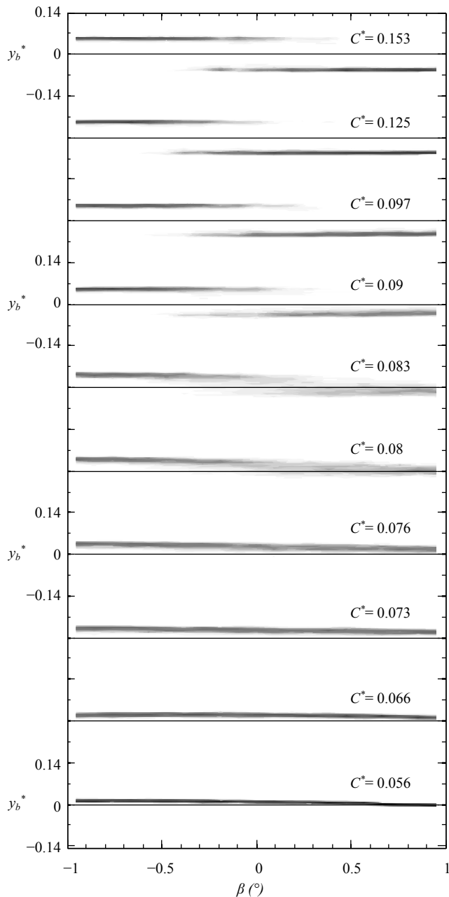
FIG. 5: Evolution of the probability density function, \text{PDF}(y_b^*) in grey levels (the darker, the larger the PDF) for U_0 = 30.58 \text{ m}\cdot\text{s}^{-1} with the yaw angle \beta and for different ground clearances C^* .
