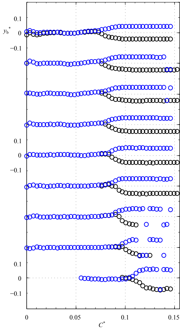
FIG. 8: Bifurcation diagrams vs. the ground clearance obtained with different Reynolds numbers, from bottom to top: Re=1.78 \times 10^4, 2.89 \times 10^4, 3.95 \times 10^4, 5.05 \times 10^4, 6.1 \times 10^4, 8.27 \times 10^4, 1.04 \times 10^5, 1.32 \times 10^5, 1.6 \times 10^5 . For each Reynolds number, the branches are extracted from the most probable position of the barycentre obtained from \beta = -0.4^\circ (blue circles) and \beta = +0.4^\circ (white circles) as in Fig. 7(a) and (b).
