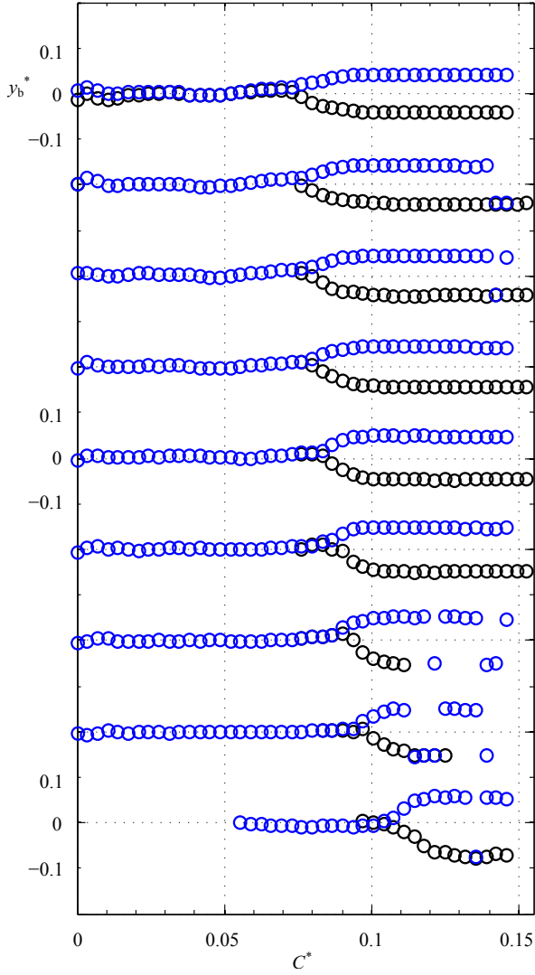
FIG. 8: Bifurcation diagrams vs. the ground clearance obtained with different Reynolds numbers, from bottom to top : Re=1.78 \times 10^4, 2.89 \times 10^4, 3.95 \times 10^4, 5.05 \times 10^4, 6.1 \times 10^4, 8.27 \times 10^4, 1.04 \times 10^5, 1.32 \times 10^5, 1.6 \times 10^5 . For each Reynolds number, the branches are extracted from the most probable position of the barycentre obtained from \beta = -0.4^\circ (blue circles) and \beta = +0.4^\circ (white circles) as in Fig. 7(a) and (b).
