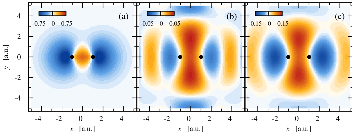
Figure 2. Highest Occupied Molecular Orbital of \text{N}_2 : (a) Hartree-Fock orbital; (b) reconstruction from experimental data; (c) reconstruction from theoretical PW dipoles filtered as in the experimental conditions. Black dots indicate the nuclei positions.
