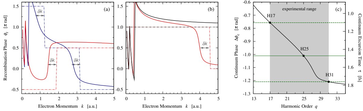
Figure 3. Phase of the recombination dipole matrix elements parallel to the laser polarization for the N_2 HOMO (a) and HOMO-1 (b) as a function of the asymptotic electron momentum k . PW/CW dipole phases are shown in dashed/solid lines for \theta = 0 (blue), 45 (red) and 90 (black) degree. Calculations for HOMO-1 are performed using the velocity form. The continuum phase difference \Delta\phi_c is shown in (c) as a function of the harmonic order. It was computed with SFA for an 800-nm laser field with intensity 1.2 \times 10^{14} \text{ W cm}^{-2} , and the binding energies for the HOMO ( -15.58 \text{ eV} ) and HOMO-1 ( -17.00 \text{ eV} ). The horizontal lines indicate the phase differences and excursion times for the first (H17), middle (H25) and last (H31) harmonics of the considered spectral range.
