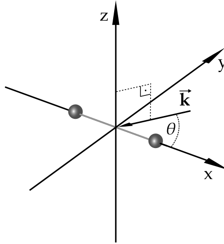
Figure 1. Reference frame for a diatomic molecule in the self-probing scheme: ( xOy ) is defined as the plane containing both the molecular axis ( Ox ) and the laser polarization direction, along which the freed EWP recollides with momentum \vec{k} . The probing orientation with respect to ( Ox ) is \theta .
