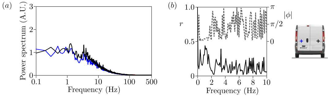
Figure 17: (a) Auto-power spectra in the lateral mixing layers from the Renault Trafic at (2.0 m, 1.0 m, 0.5 m) (black line), (2.0 m, 1.0 m, -0.5 m) (blue line). (b) Correlation (left scale, continuous line) and phase (right scale, dashed line) between the velocity signals at (2.0 m, 1.0 m, 0.5 m) and (2.0 m, 1.0 m, -0.5 m).
