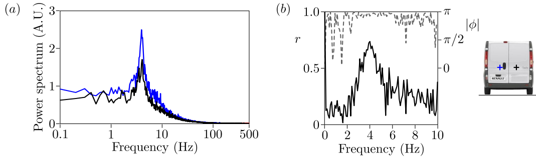
Figure 14: (a) Auto-power spectra in the lateral mixing layers from the Renault Trafic at (4.0 m, 1.0 m, 0.3 m) (black line), (4.0 m, 1.0 m, -0.3 m) (blue line). (b) Correlation (left scale, continuous line) and phase (right scale, dashed line) between the velocity signals at (4.0 m, 1.0 m, 0.3 m) and (4.0 m, 1.0 m, -0.3 m).
