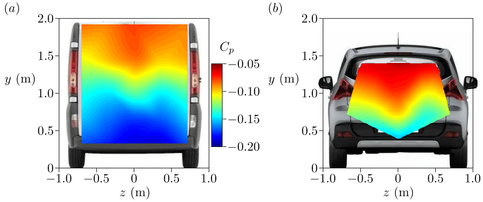
Figure 5: Distribution of static pressure on the base of the Renault Traffic (a) and of the Peugeot 3008 (b).
