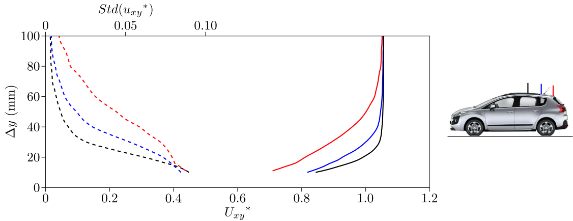
Figure 3: Mean (continuous lines) and fluctuating (dashed lines) velocity profiles of the boundary layer on the roof of the Peugeot 3008 in the plane z = 0.12 m: \Delta x = -1.0 m, black lines; \Delta x = -0.5 m, blue lines; \Delta x = -0.05 m, red lines. \Delta x and \Delta y are respectively the algebraic distances to the roof end and to the roof surface.
