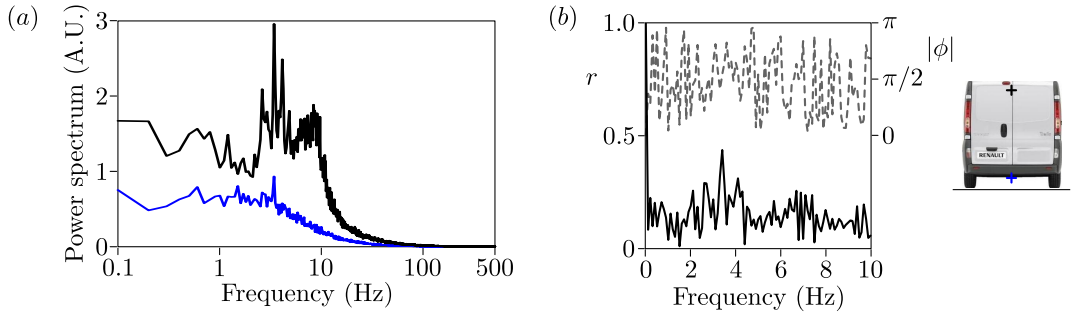
Figure 16: (a) Auto-power spectra in the top and bottom mixing layers from the Renault Trafic at (2.0 m, 1.8 m, 0 m) (black line), (2.0 m, 0.2 m, 0 m) (blue line). (b) Correlation (left scale, continuous line) and phase (right scale, dashed line) between the velocity signals at (2.0 m, 1.8 m, 0 m) and (2.0 m, 0.2 m, 0 m).
