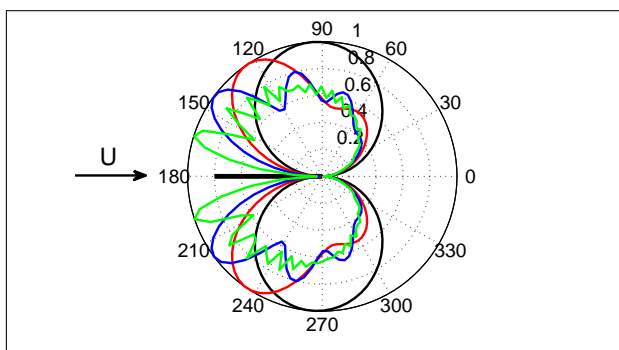
Figure 9. Directivity of trailing edge noise predicted by Amiet's model at 16 Hz (black), 50 Hz (red), 120 Hz (blue) and 500 Hz (green). The flat plate is represented in black.
