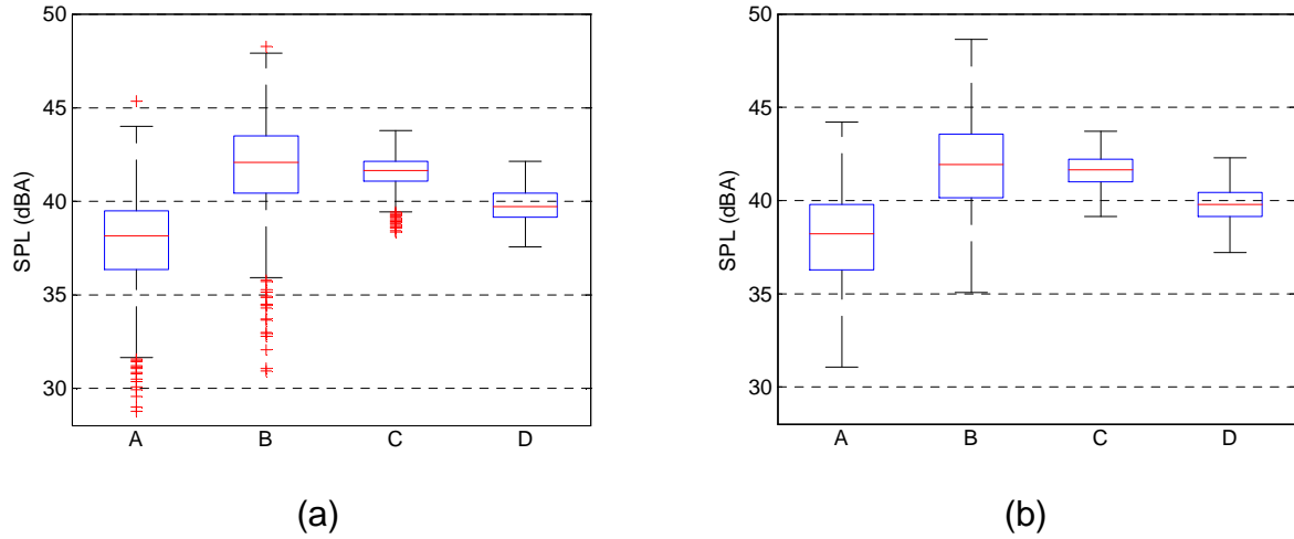
Figure 8 : Box plots of SPL for the four selected periods using (a) reference data, and (b) Monte Carlo simulations with N = 10\,000 . Outliers are shown only for reference data.
