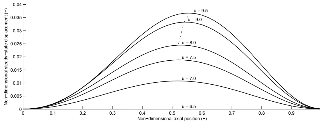
Figure 9: Simulated steady-state displacement of the buckled cylinder at different flow velocities with indication of the downstream shift of the maximal displacement.
