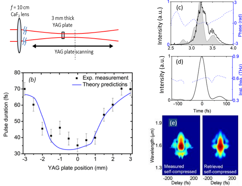
Fig. 7 (a) Layout of the self-compression setup. The input beam is focused by a 10 cm focal length CaF 2 lens into a 3 mm-thick YAG plate. The YAG plate is moved along the beam propagation axis, through focus. (b) measured (black dots) and simulated (blue line) evolution of the pulse duration as a function of YAG plate position through focus. (c) Measured (black line) and retrieved (shadow) spectra of the self-compressed pulses. (d) Retrieved normalized 32 fs (2.9-cycle) duration intensity profile of the self-compressed pulses. (e) Measured and retrieved SHG-FROG traces of the self-compressed pulses on logarithmic color scale. Adapted from [15].
