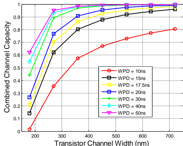
Fig. 22. STT-MRAM written-in bits (WIBs) distributions with different transistor widths and different WPDs (RPD = 5ns).
