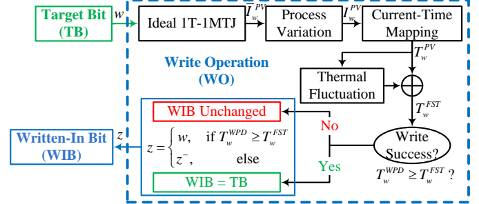
Fig.3. Block diagram of the write operation channel.
