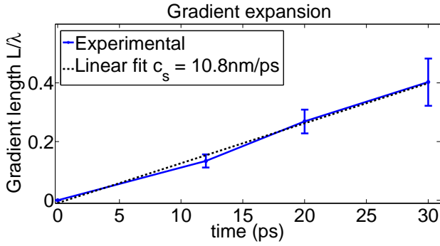
Fig. 3. Measured relative plasma expansion velocity for a pump pulse intensity of I_{p,1} = 3.5 \times 10^{14} \text{ W/cm}^2 as a function of pump-probe delay. Each experimental point corresponds to an inversion in the far-field probe beam intensity profile induced by the expanding critical surface of the plasma formed at the surface of the solid target. Inversions are defined by \Delta\phi = n\pi with here n = 0, 1, 2, 3 .
