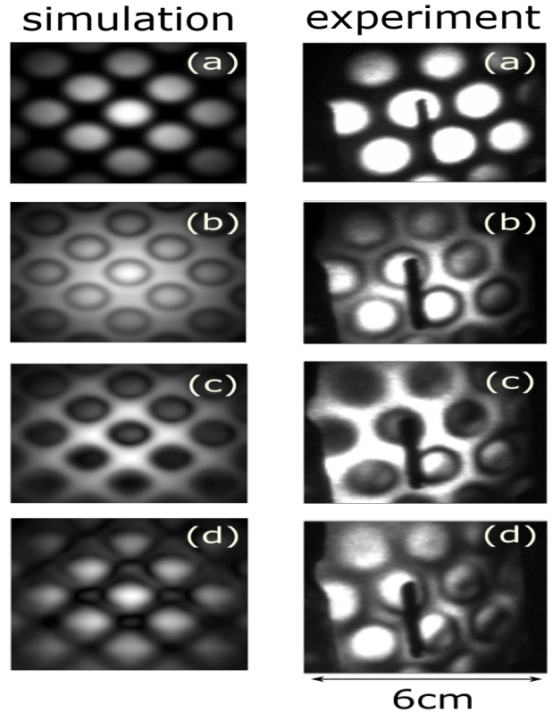
Fig. 2. Simulated (left column) and experimental (right column) far-field probe beam intensity profile inversions at respectively 0 ps(a) 6 ps(b), 12 ps(c) and 20 ps(d) pump-probe delay. The visible shadow is an experimental artefact. The simulations are performed using the measured pump beam profile and assuming the plasma expansion velocity to be proportional to the square root of the pump pulse intensity. The corresponding phase shifts in Rad are respectively 0(a), \pi/2 (b), \pi (c) and 2\pi (d)
