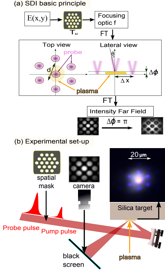
Fig. 1. (a) : SDI principle applied to ultrafast plasma mirror imaging: the probe field E(x, y) is diffracted by an intensity mask T_M onto a plasma mirror in the focal plane. The phase shift, \Delta\phi , of the central diffraction spot induced by the plasma expansion leads to an inversion of the far-field spatial intensity profile of the reflected probe beam for \Delta\phi = \pi (b) : Experimental set-up: a 30 fs pump pulse is focused onto a solid target using an off-axis parabola in order to induce a plasma mirror. The far-field intensity profile of the time-delayed spatially shaped probe pulse reflected by the plasma mirror is imaged onto a CCD camera and recorded as a function of pump-probe delay. The far right panel shows both pump (gray scale) and probe (color scale) beam profiles measured at focus on target.
