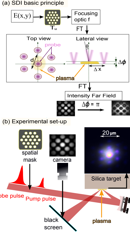
Fig. 1. (a) : SDI principle applied to ultrafast plasma mirror imaging: the probe field E(x,y) is diffracted by an intensity mask T_M onto a plasma mirror in the focal plane. The phase shift, \Delta\phi , of the central diffraction spot induced by the plasma expansion leads to an inversion of the far-field spatial intensity profile of the reflected probe beam for \Delta\phi = \pi (b) : Experimental set-up: a 30 fs pump pulse is focused onto a solid target using an off-axis parabola in order to induce a plasma mirror. The far-field intensity profile of the time-delayed spatially shaped probe pulse reflected by the plasma mirror is imaged onto a CCD camera and recorded as a function of pump-probe delay. The far right panel shows both pump (gray scale) and probe (color scale) beam profiles measured at focus on target.
