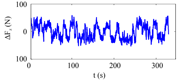
Figure 10 Lift time series for \beta = +4^\circ .
