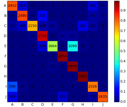
Fig. 5. Confusion matrix for the standard MLP.
