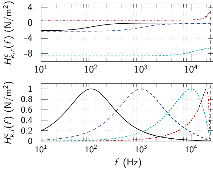
Figure 3: H_{k,r}^c and H_{k,i}^c for values of p_k satisfying (6) and H_{0k}p_k \leq 0 ( f_s = 48 kHz): p_k = 0.99 (—), p_k = 0.88 (---), p_k = 0.13 (- · -) and p_k = -0.58 (· · ·). The vertical dashed line corresponds to f_s/2 .
