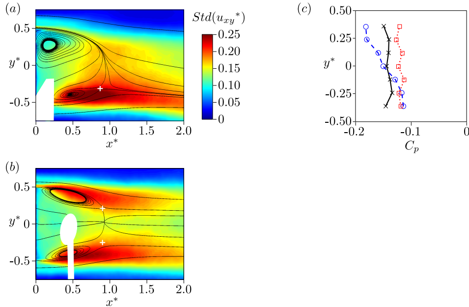
Figure 11: Streamlines in the plane z^* = 0 for the controlled case x_C^* = 0.2 and y_C^* = -0.3 (a) and x_C^* = 0.5 and y_C^* = 0 (b) ; colormap of the fluctuating velocities ; white cross, collar point. (c) Base pressure distribution: — ( \times ), natural flow ; -- ( \circ ), x_C^* = 0.2 and y_C^* = -0.3 (see Fig. 11(a)) ; \cdot\cdot ( \square ), x_C^* = 0.5 and y_C^* = 0 (see Fig. 11(b)).
