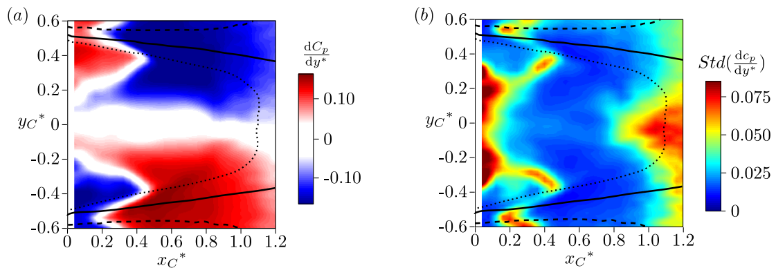
Figure 8: Effect of the position of the 3 mm control cylinder on dC_p/dy^* (a) and on Std(dC_p/dy^*) (b); contours of U_x^* for the natural flow: \cdot\cdot , 0.1; — , 0.5; -- , 0.9.
