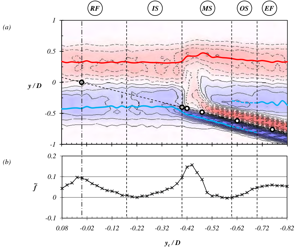
FIGURE 20. (a) Mean vorticity sequence \bar{\omega}_z(y, x = 0.44D, y_c) , for the 3mm control cylinder, showing the vertical vorticity distribution across the wake downstream of the control cylinder ( x_c = 0.44D, y_c ). The contours of vorticity are the same as in figure 8(b). The dashed line denotes the path of the control cylinder across the wake, and circles represent the positions of the control cylinder presented in figure 8 and figure 10. Diagram (b) shows frequency \tilde{f} of the global mode. Notation RF , IS , MS , OS and EF refers to configurations defined in section 3.2.2.
