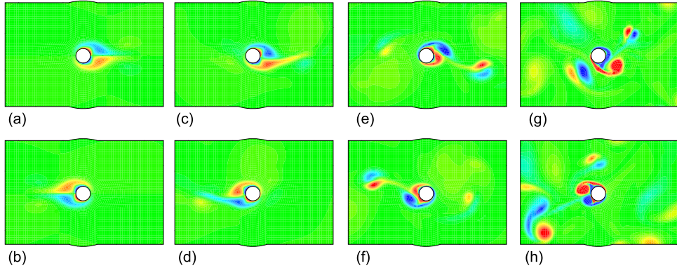
Fig. 8. Vorticity field around the cylinder at two consecutive half-cycles for the four dominant modes observed for KC=10 and 40 \leq Re \leq 500 . The color bar is between -4 and +4 for every sub-figure. (a) Re=60 at t=109.45T representative of 40 \leq Re \leq 70 (regime A), (b) Re=60 at t=109.95T representative of 40 \leq Re \leq 70 (regime A), (c) Re=90 at t=149.45T representative of 80 \leq Re \leq 100 (regime D), (d) Re=90 at t=149.95T representative of 80 \leq Re \leq 100 (regime D), (e) Re=170 at t=99.45T representative of 110 \leq Re \leq 280 (regime F), (f) Re=170 at t=99.95T representative of 110 \leq Re \leq 280 (regime F), (g) Re=360 at t=34.45T representative of 320 \leq Re \leq 500 (regime G) and (h) Re=360 at t=34.95T representative of 320 \leq Re \leq 500 (regime G). (For interpretation of the references to color in this figure legend, the reader is referred to the web version of this article.)
